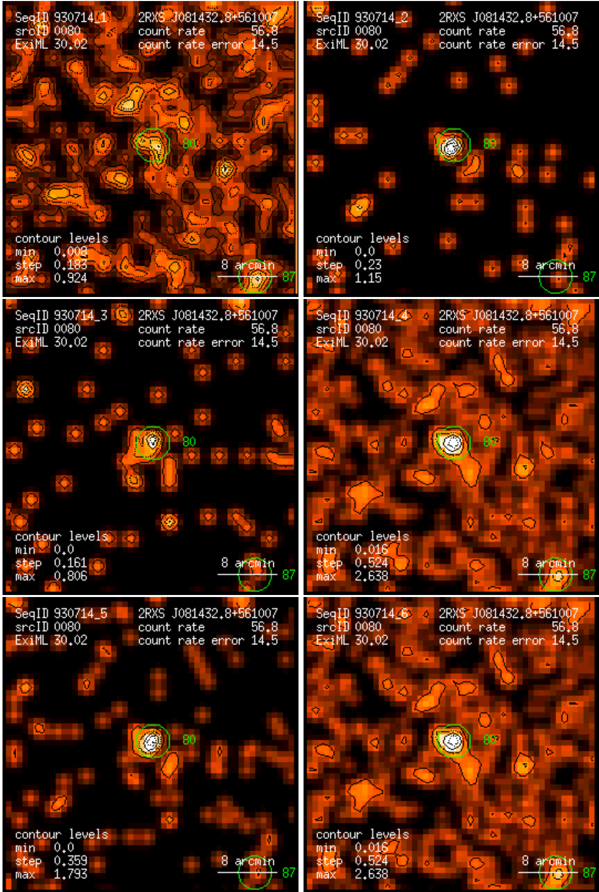
Figure 80: RASS 930714: detection 0080: band rate images, Gaussian filter: (1) PSPC channels 11 – 41, (2) 52 – 90, (3) 91 – 201, (4) 11 – 235, (5) 52 – 201, (6) 11 – 201. Broad band rates in counts/ks. Band rate contour levels in counts/ks/arcmin 2 .
