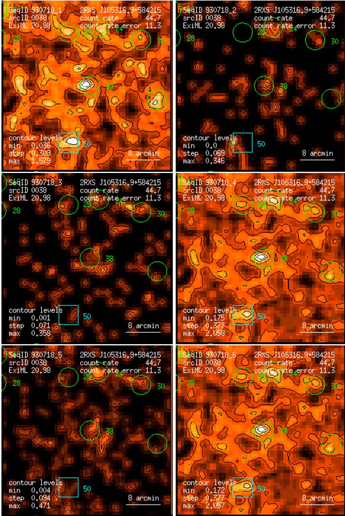
Figure 38: RASS 930718: detection 0038: band rate images, Gaussian filter: (1) PSPC channels 11 – 41, (2) 52 – 90, (3) 91 – 201, (4) 11 – 235, (5) 52 – 201, (6) 11 – 201. Broad band rates in counts/ks. Band rate contour levels in counts/ks/arcmin 2 .
