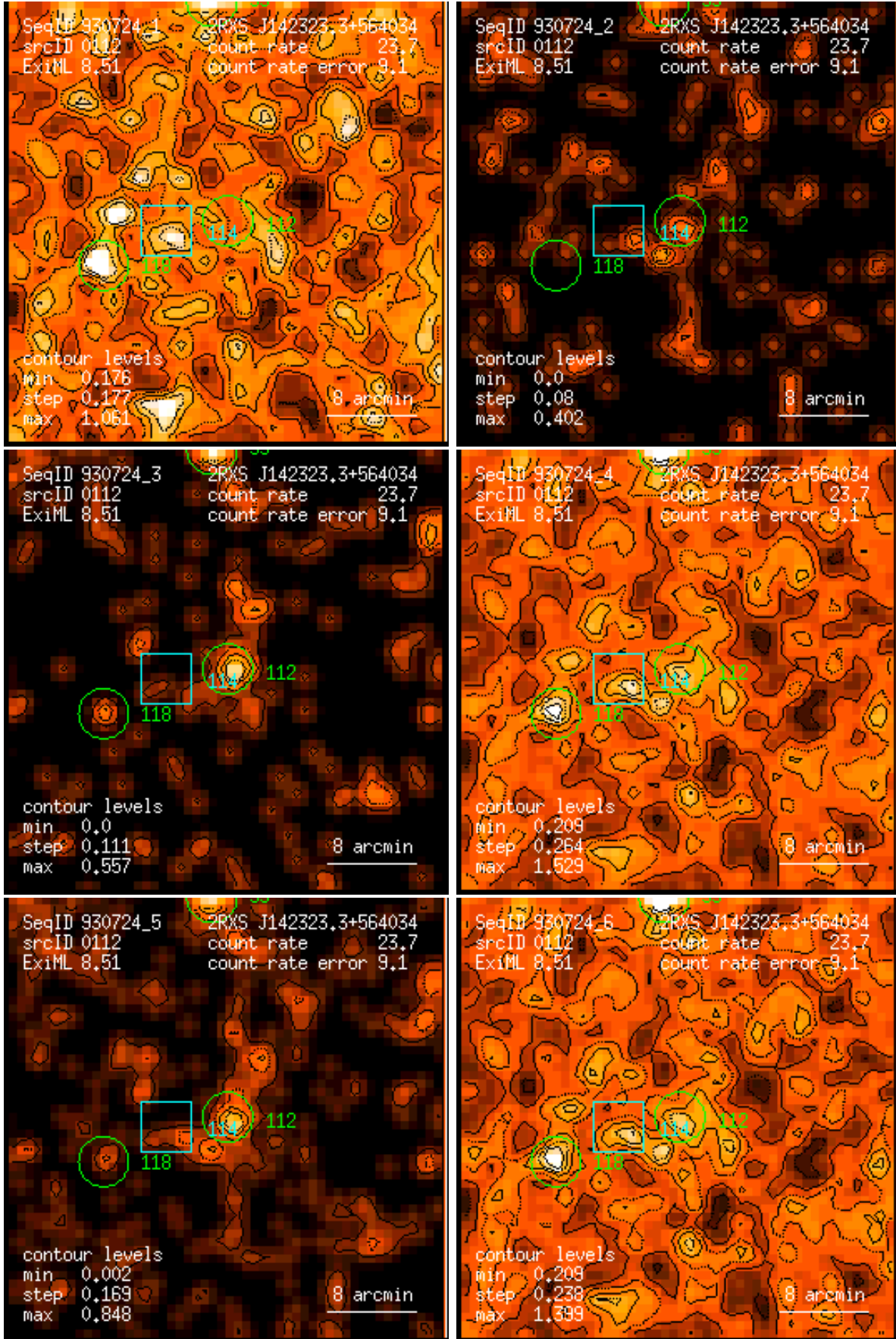
Figure 112: RASS 930724: detection 0112: band rate images, Gaussian filter: (1) PSPC channels 11 – 41, (2) 52 – 90, (3) 91 – 201, (4) 11 – 235, (5) 52 – 201, (6) 11 – 201. Broad band rates in counts/ks. Band rate contour levels in counts/ks/arcmin 2 .
