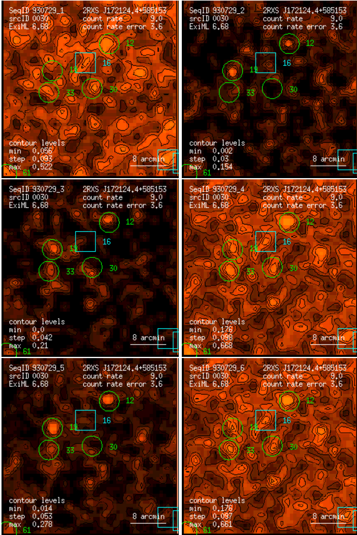
Figure 30: RASS 930729: detection 0030: band rate images, Gaussian filter: (1) PSPC channels 11 – 41, (2) 52 – 90, (3) 91 – 201, (4) 11 – 235, (5) 52 – 201, (6) 11 – 201. Broad band rates in counts/ks. Band rate contour levels in counts/ks/arcmin 2 .
