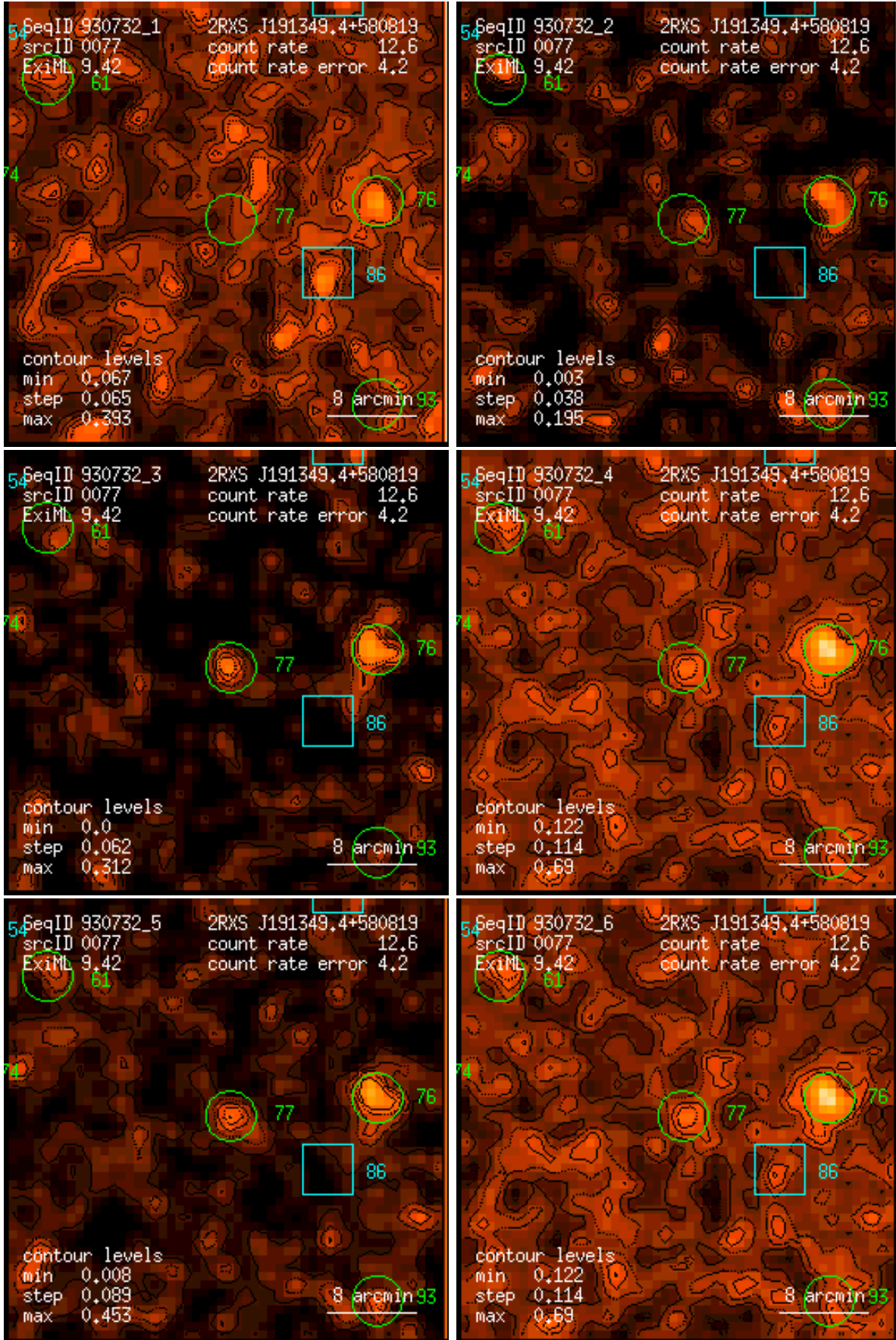
Figure 77: RASS 930732: detection 0077: band rate images, Gaussian filter: (1) PSPC channels 11 – 41, (2) 52 – 90, (3) 91 – 201, (4) 11 – 235, (5) 52 – 201, (6) 11 – 201. Broad band rates in counts/ks. Band rate contour levels in counts/ks/arcmin 2 .
