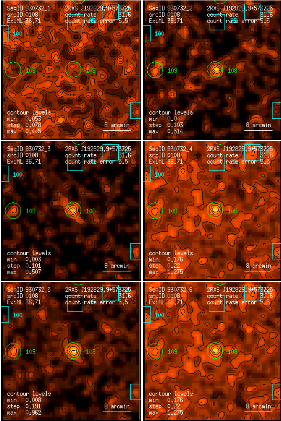
Figure 108: RASS 930732: detection 0108: band rate images, Gaussian filter: (1) PSPC channels 11 – 41, (2) 52 – 90, (3) 91 – 201, (4) 11 – 235, (5) 52 – 201, (6) 11 – 201. Broad band rates in counts/ks. Band rate contour levels in counts/ks/arcmin 2 .
