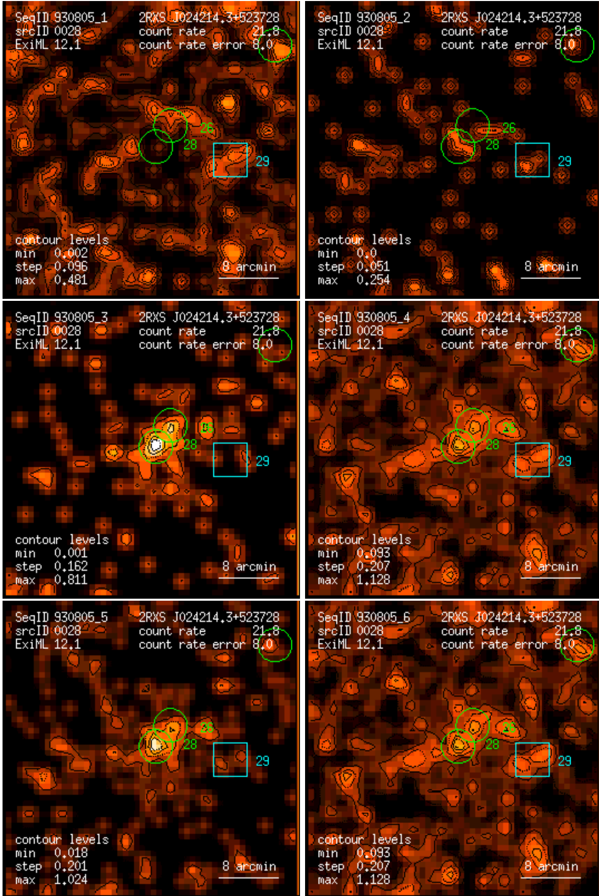
Figure 28: RASS 930805: detection 0028: band rate images, Gaussian filter: (1) PSPC channels 11 – 41, (2) 52 – 90, (3) 91 – 201, (4) 11 – 235, (5) 52 – 201, (6) 11 – 201. Broad band rates in counts/ks. Band rate contour levels in counts/ks/arcmin 2 .
