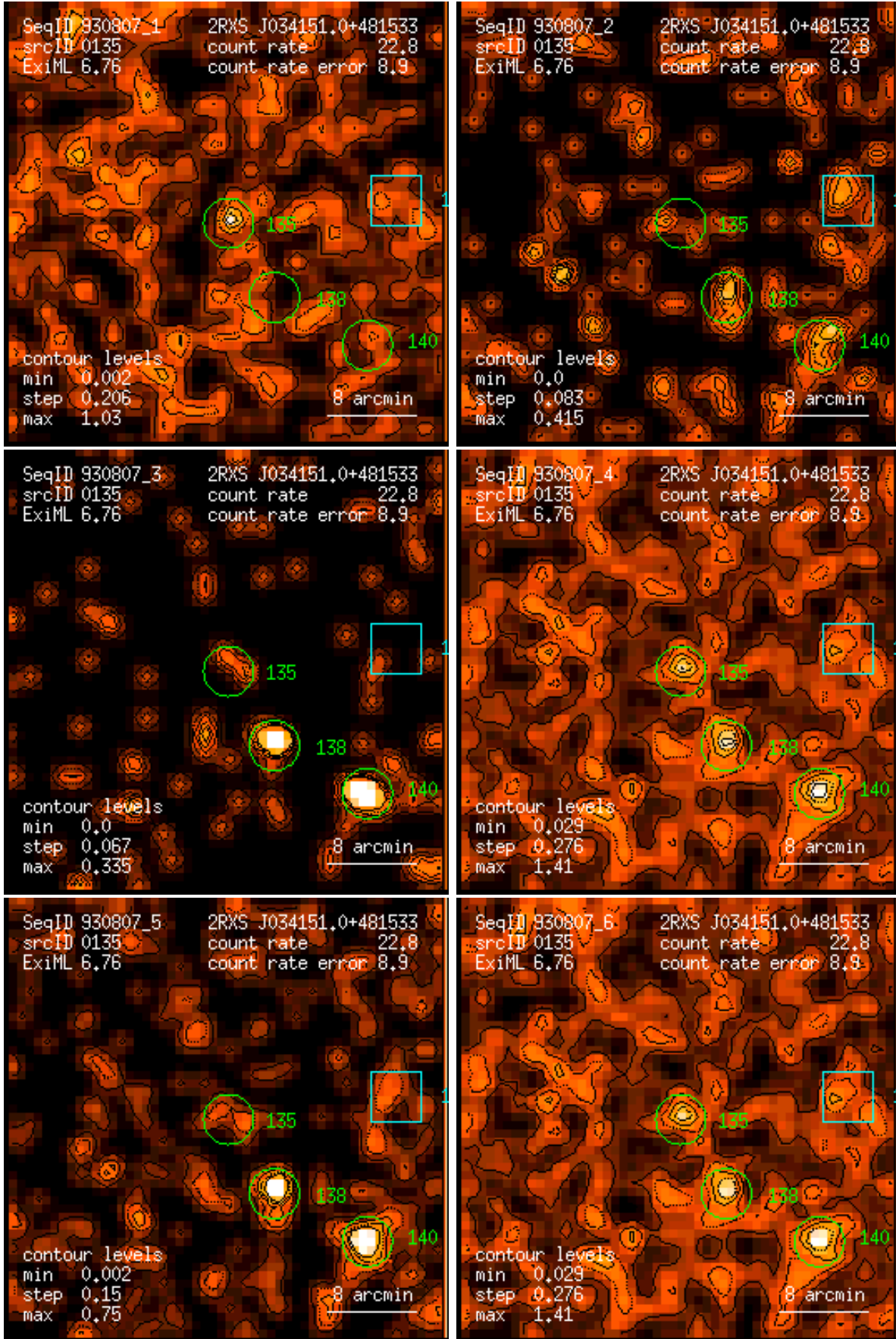
Figure 135: RASS 930807: detection 0135: band rate images, Gaussian filter: (1) PSPC channels 11 – 41, (2) 52 – 90, (3) 91 – 201, (4) 11 – 235, (5) 52 – 201, (6) 11 – 201. Broad band rates in counts/ks. Band rate contour levels in counts/ks/arcmin 2 .
