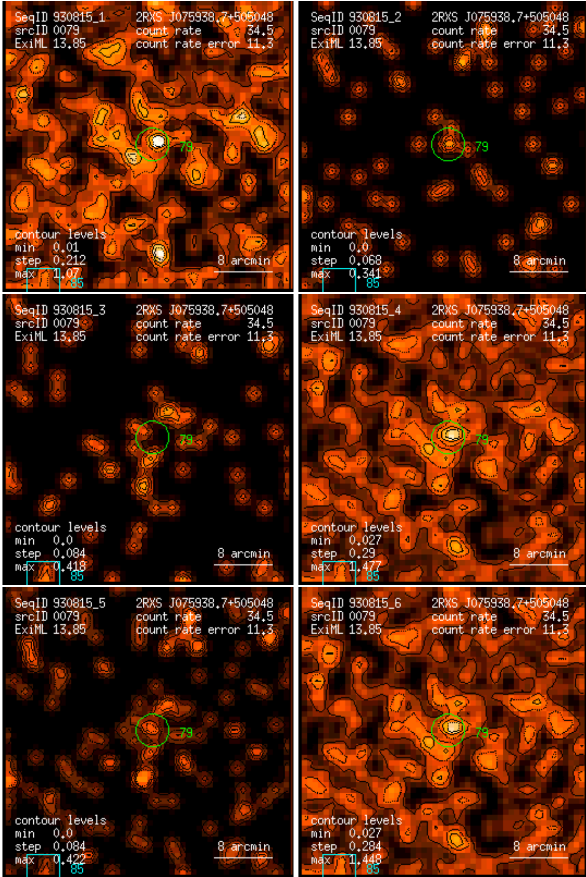
Figure 79: RASS 930815: detection 0079: band rate images, Gaussian filter: (1) PSPC channels 11 – 41, (2) 52 – 90, (3) 91 – 201, (4) 11 – 235, (5) 52 – 201, (6) 11 – 201. Broad band rates in counts/ks. Band rate contour levels in counts/ks/arcmin 2 .
