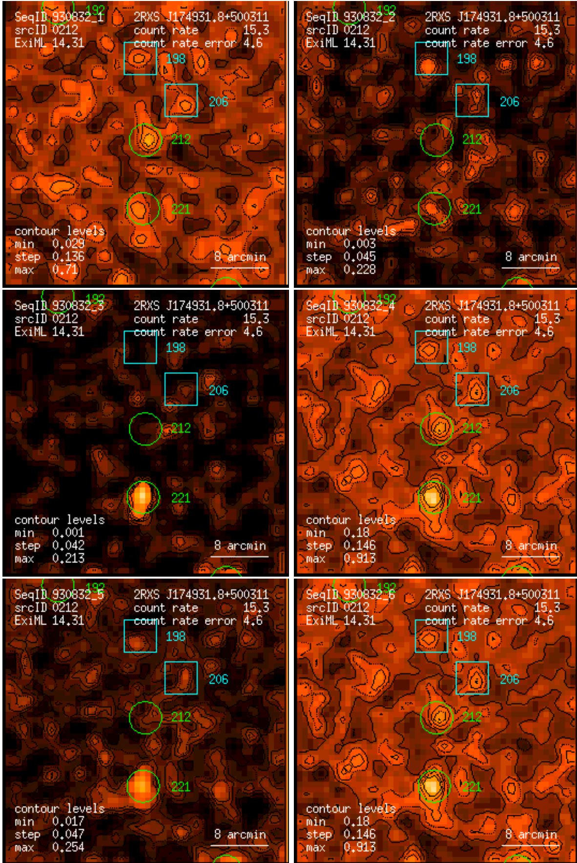
Figure 212: RASS 930832: detection 0212: band rate images, Gaussian filter: (1) PSPC channels 11 – 41, (2) 52 – 90, (3) 91 – 201, (4) 11 – 235, (5) 52 – 201, (6) 11 – 201. Broad band rates in counts/ks. Band rate contour levels in counts/ks/arcmin 2 .
