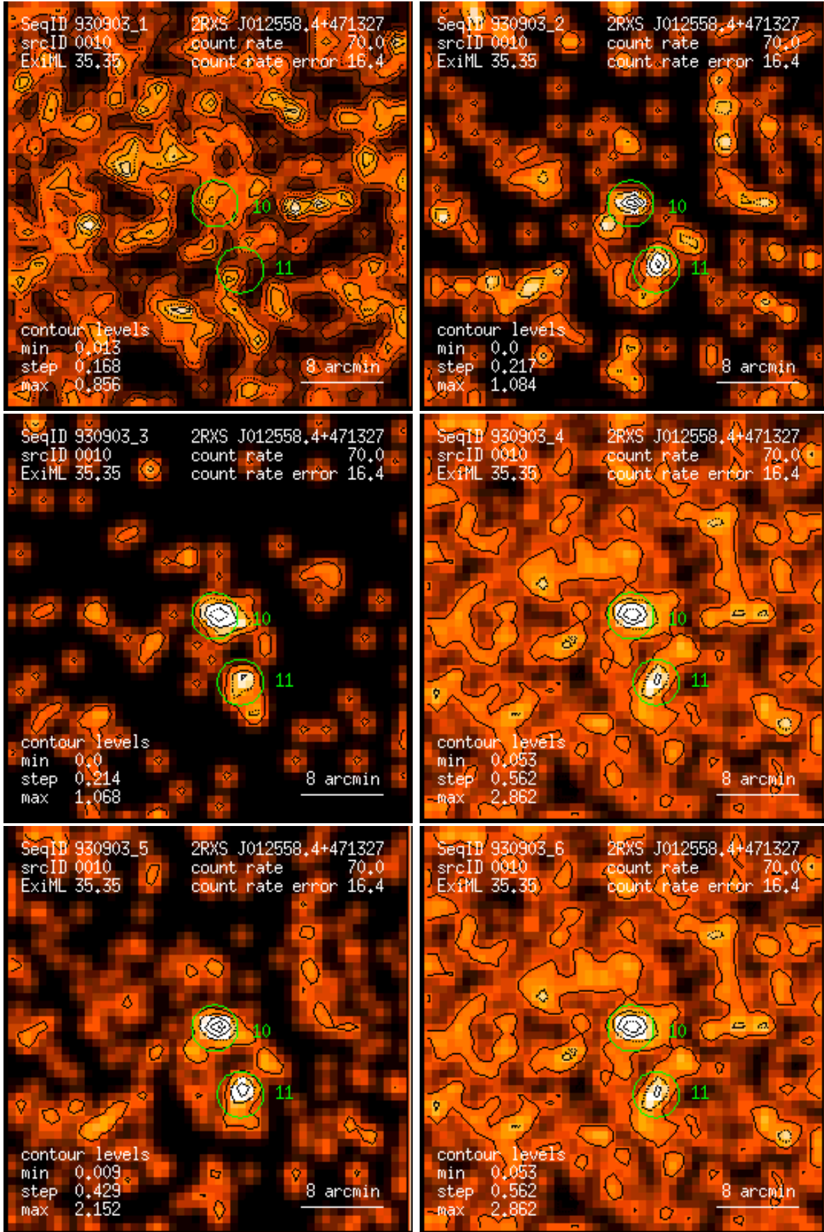
Figure 10: RASS 930903: detection 0010: band rate images, Gaussian filter: (1) PSPC channels 11 – 41, (2) 52 – 90, (3) 91 – 201, (4) 11 – 235, (5) 52 – 201, (6) 11 – 201. Broad band rates in counts/ks. Band rate contour levels in counts/ks/arcmin 2 .
