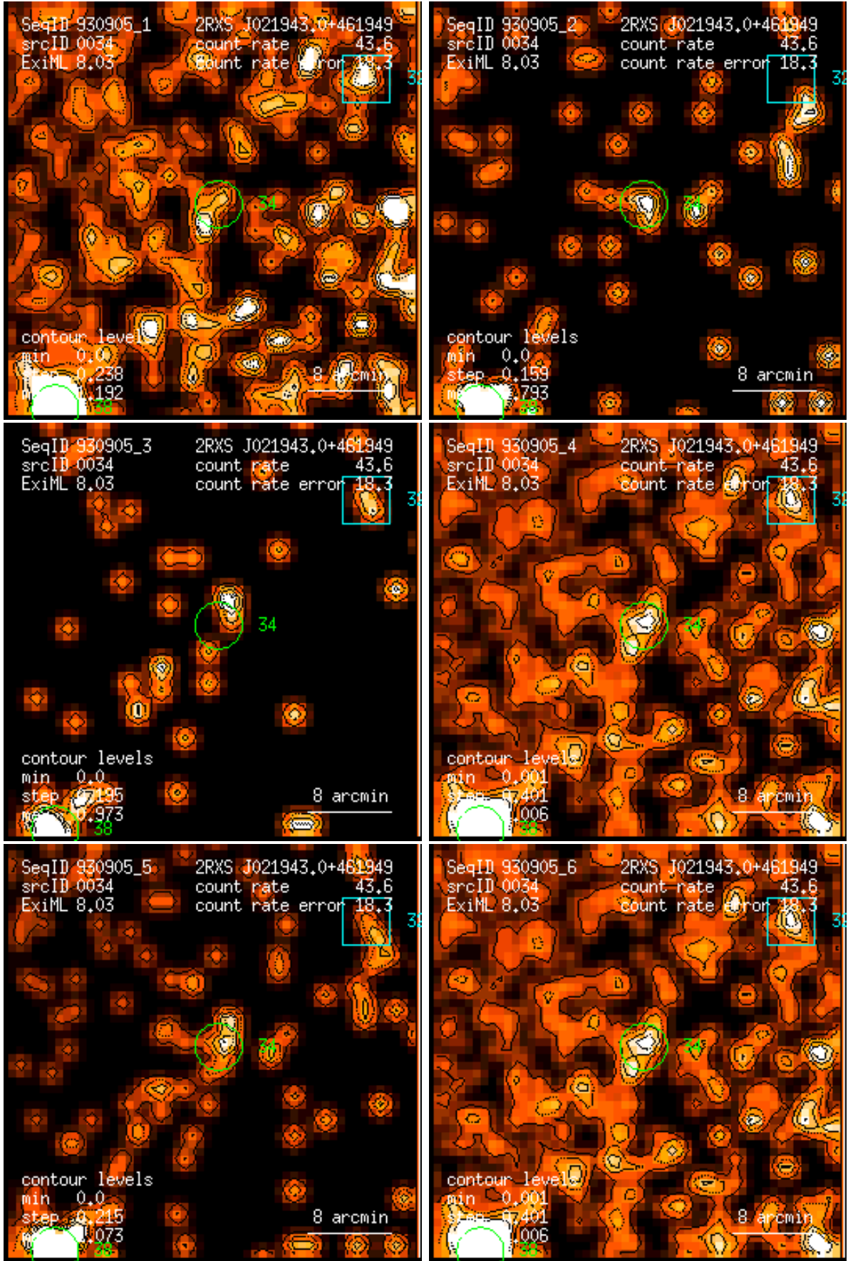
Figure 34: RASS 930905: detection 0034: band rate images, Gaussian filter: (1) PSPC channels 11 – 41, (2) 52 – 90, (3) 91 – 201, (4) 11 – 235, (5) 52 – 201, (6) 11 – 201. Broad band rates in counts/ks. Band rate contour levels in counts/ks/arcmin 2 .
