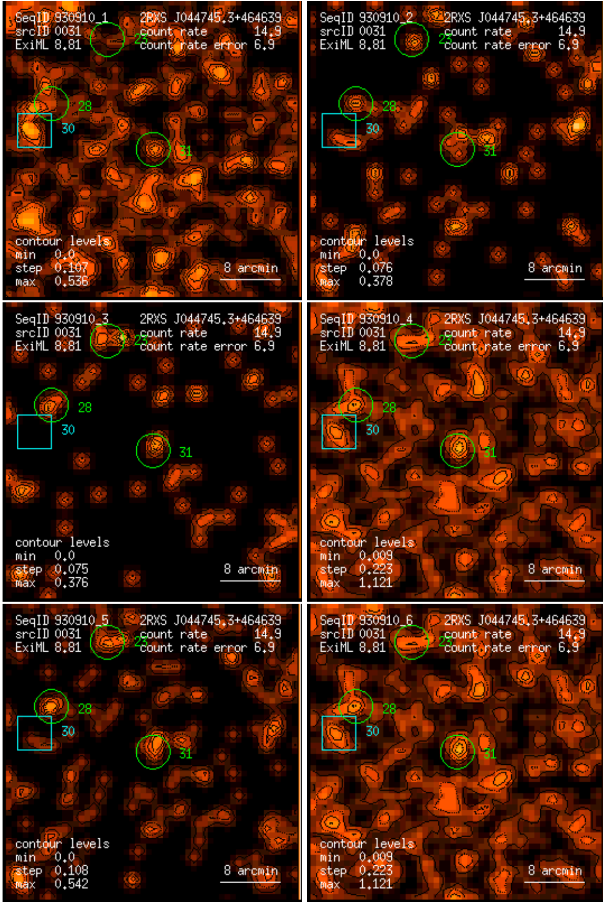
Figure 31: RASS 930910: detection 0031: band rate images, Gaussian filter: (1) PSPC channels 11 – 41, (2) 52 – 90, (3) 91 – 201, (4) 11 – 235, (5) 52 – 201, (6) 11 – 201. Broad band rates in counts/ks. Band rate contour levels in counts/ks/arcmin 2 .
