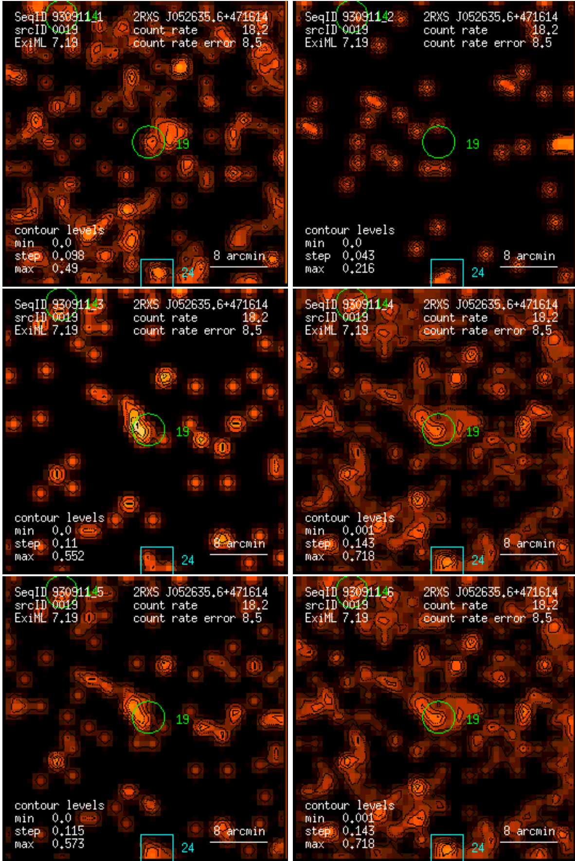
Figure 19: RASS 930911: detection 0019: band rate images, Gaussian filter: (1) PSPC channels 11 – 41, (2) 52 – 90, (3) 91 – 201, (4) 11 – 235, (5) 52 – 201, (6) 11 – 201. Broad band rates in counts/ks. Band rate contour levels in counts/ks/arcmin 2 .
