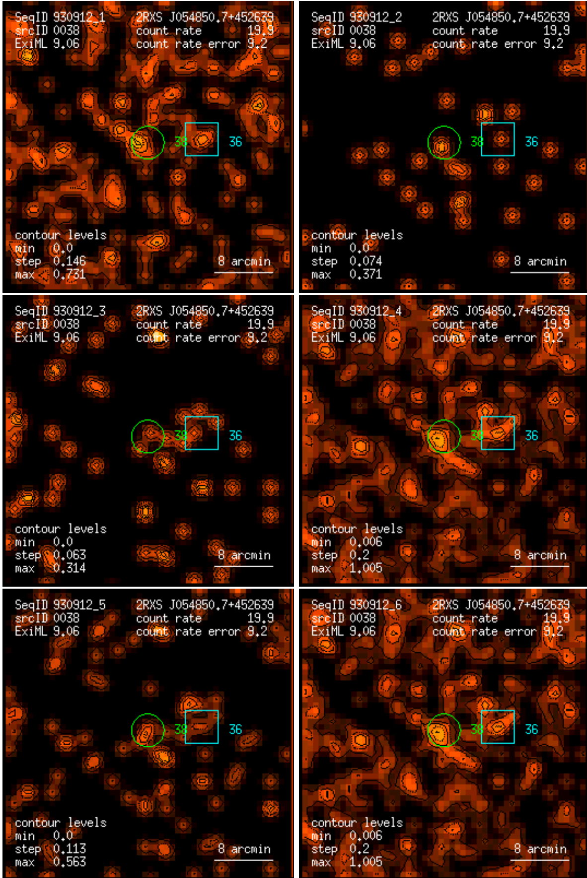
Figure 38: RASS 930912: detection 0038: band rate images, Gaussian filter: (1) PSPC channels 11 – 41, (2) 52 – 90, (3) 91 – 201, (4) 11 – 235, (5) 52 – 201, (6) 11 – 201. Broad band rates in counts/ks. Band rate contour levels in counts/ks/arcmin 2 .
