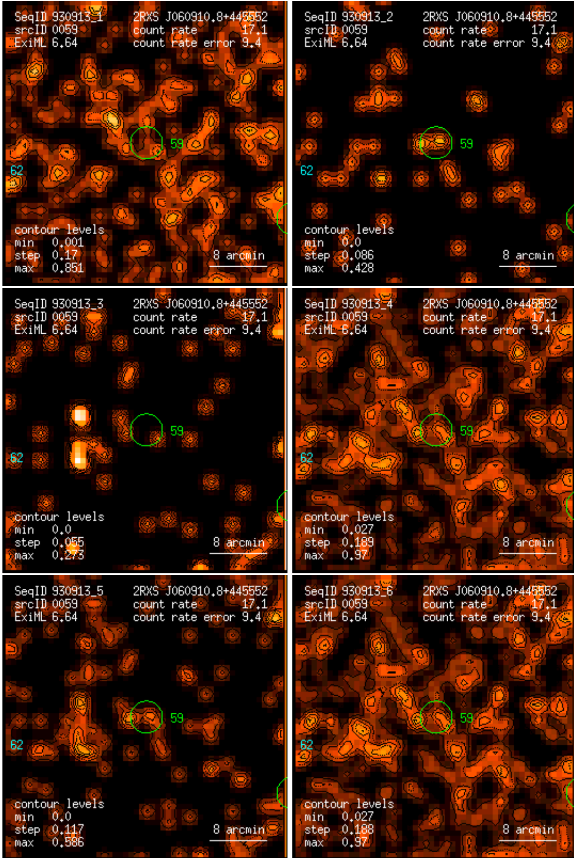
Figure 59: RASS 930913: detection 0059: band rate images, Gaussian filter: (1) PSPC channels 11 – 41, (2) 52 – 90, (3) 91 – 201, (4) 11 – 235, (5) 52 – 201, (6) 11 – 201. Broad band rates in counts/ks. Band rate contour levels in counts/ks/arcmin 2 .
