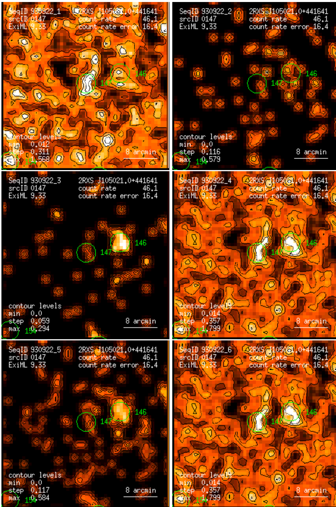
Figure 147: RASS 930922: detection 0147: band rate images, Gaussian filter: (1) PSPC channels 11 – 41, (2) 52 – 90, (3) 91 – 201, (4) 11 – 235, (5) 52 – 201, (6) 11 – 201. Broad band rates in counts/ks. Band rate contour levels in counts/ks/arcmin 2 .
