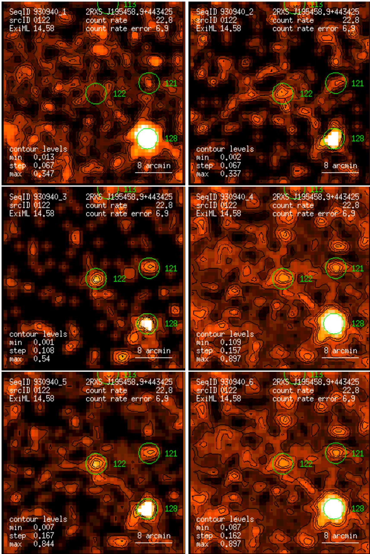
Figure 122: RASS 930940: detection 0122: band rate images, Gaussian filter: (1) PSPC channels 11 – 41, (2) 52 – 90, (3) 91 – 201, (4) 11 – 235, (5) 52 – 201, (6) 11 – 201. Broad band rates in counts/ks. Band rate contour levels in counts/ks/arcmin 2 .
