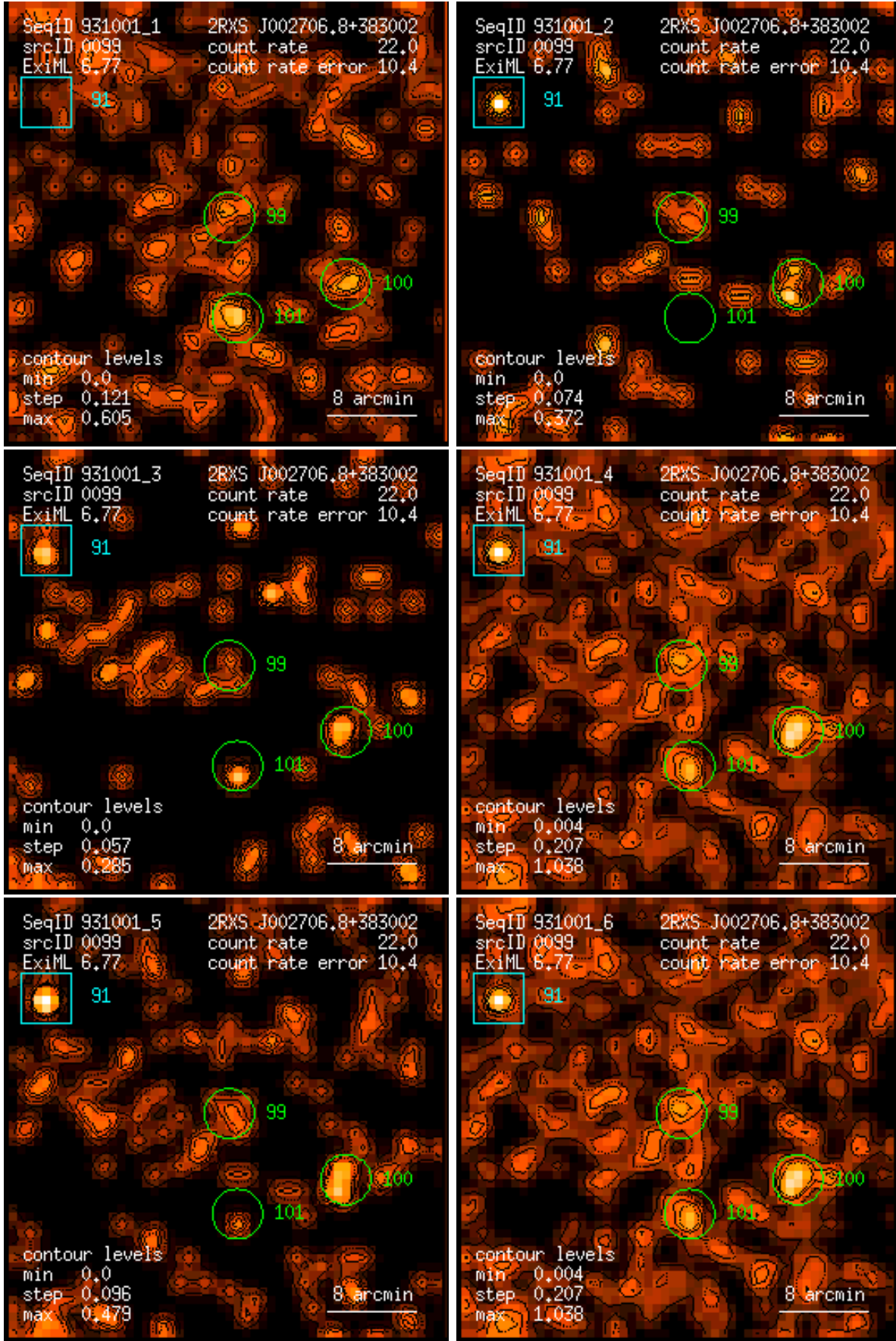
Figure 99: RASS 931001: detection 0099: band rate images, Gaussian filter: (1) PSPC channels 11 – 41, (2) 52 – 90, (3) 91 – 201, (4) 11 – 235, (5) 52 – 201, (6) 11 – 201. Broad band rates in counts/ks. Band rate contour levels in counts/ks/arcmin 2 .
