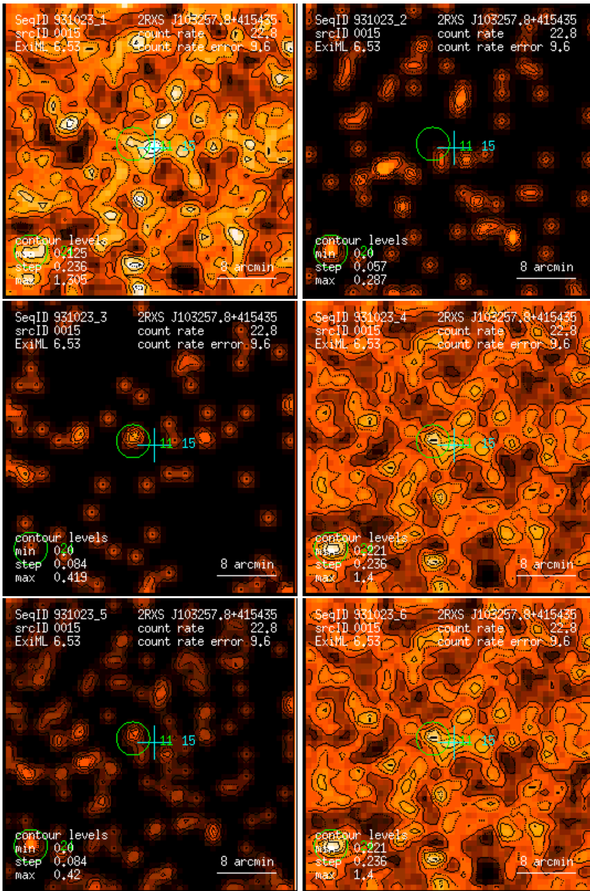
Figure 15: RASS 931023: detection 0015: band rate images, Gaussian filter: (1) PSPC channels 11 – 41, (2) 52 – 90, (3) 91 – 201, (4) 11 – 235, (5) 52 – 201, (6) 11 – 201. Broad band rates in counts/ks. Band rate contour levels in counts/ks/arcmin 2 .
