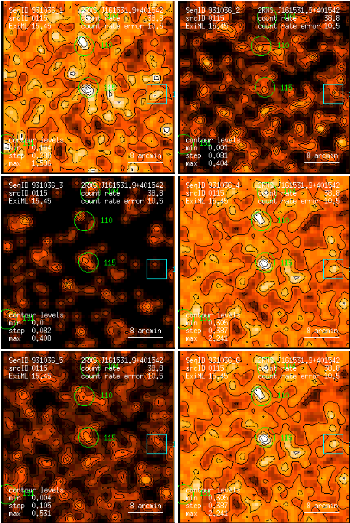
Figure 115: RASS 931036: detection 0115: band rate images, Gaussian filter: (1) PSPC channels 11 – 41, (2) 52 – 90, (3) 91 – 201, (4) 11 – 235, (5) 52 – 201, (6) 11 – 201. Broad band rates in counts/ks. Band rate contour levels in counts/ks/arcmin 2 .
