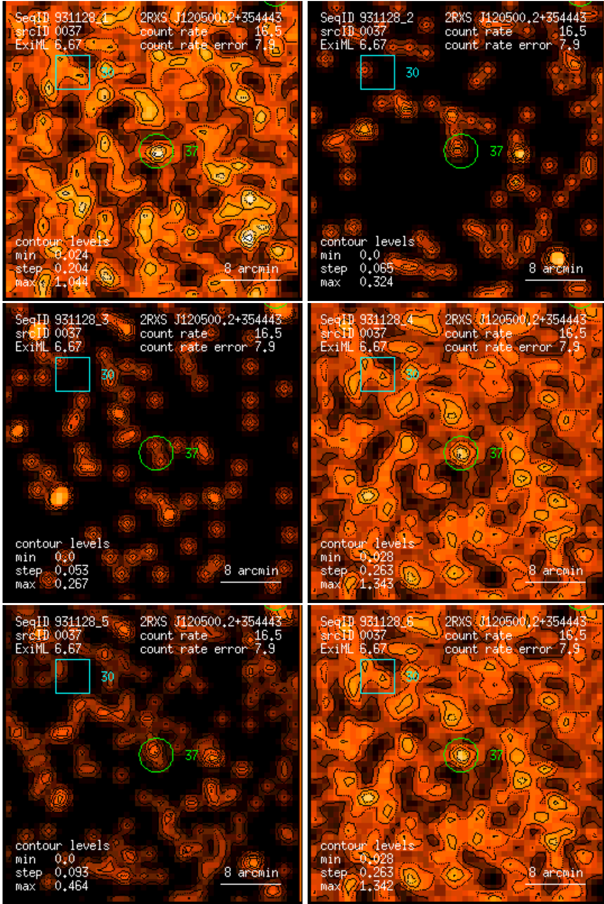
Figure 37: RASS 931128: detection 0037: band rate images, Gaussian filter: (1) PSPC channels 11 – 41, (2) 52 – 90, (3) 91 – 201, (4) 11 – 235, (5) 52 – 201, (6) 11 – 201. Broad band rates in counts/ks. Band rate contour levels in counts/ks/arcmin 2 .
