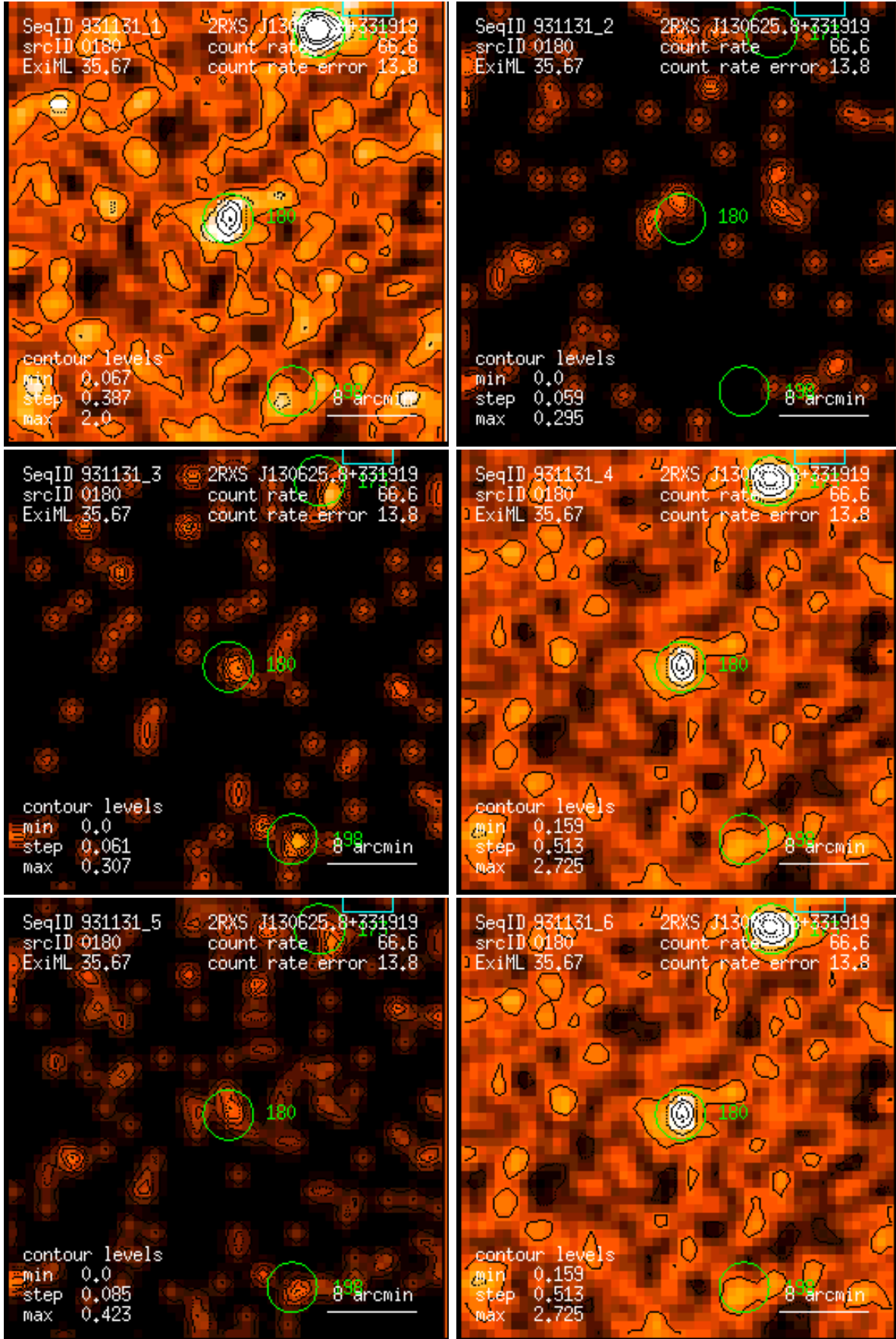
Figure 180: RASS 931131: detection 0180: band rate images, Gaussian filter: (1) PSPC channels 11 – 41, (2) 52 – 90, (3) 91 – 201, (4) 11 – 235, (5) 52 – 201, (6) 11 – 201. Broad band rates in counts/ks. Band rate contour levels in counts/ks/arcmin 2 .
