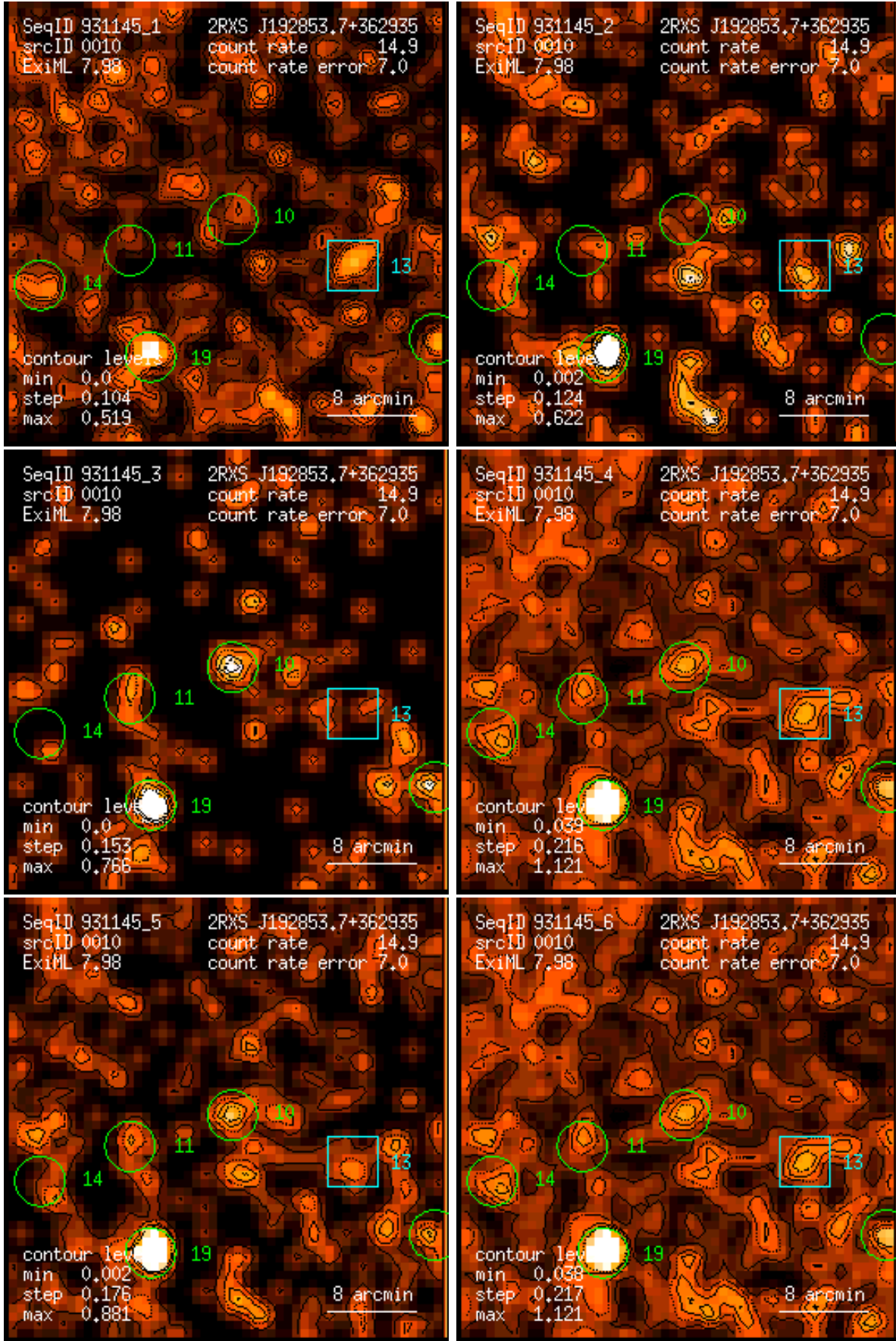
Figure 10: RASS 931145: detection 0010: band rate images, Gaussian filter: (1) PSPC channels 11 – 41, (2) 52 – 90, (3) 91 – 201, (4) 11 – 235, (5) 52 – 201, (6) 11 – 201. Broad band rates in counts/ks. Band rate contour levels in counts/ks/arcmin 2 .
