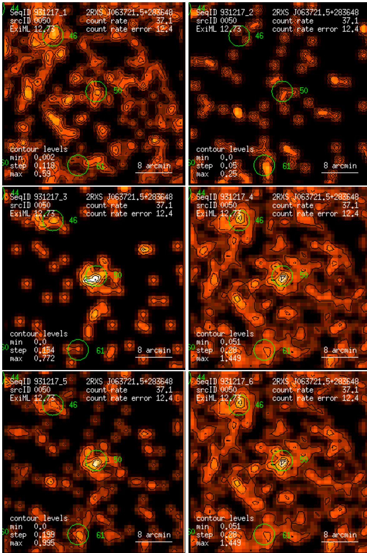
Figure 50: RASS 931217: detection 0050: band rate images, Gaussian filter: (1) PSPC channels 11 – 41, (2) 52 – 90, (3) 91 – 201, (4) 11 – 235, (5) 52 – 201, (6) 11 – 201. Broad band rates in counts/ks. Band rate contour levels in counts/ks/arcmin 2 .
