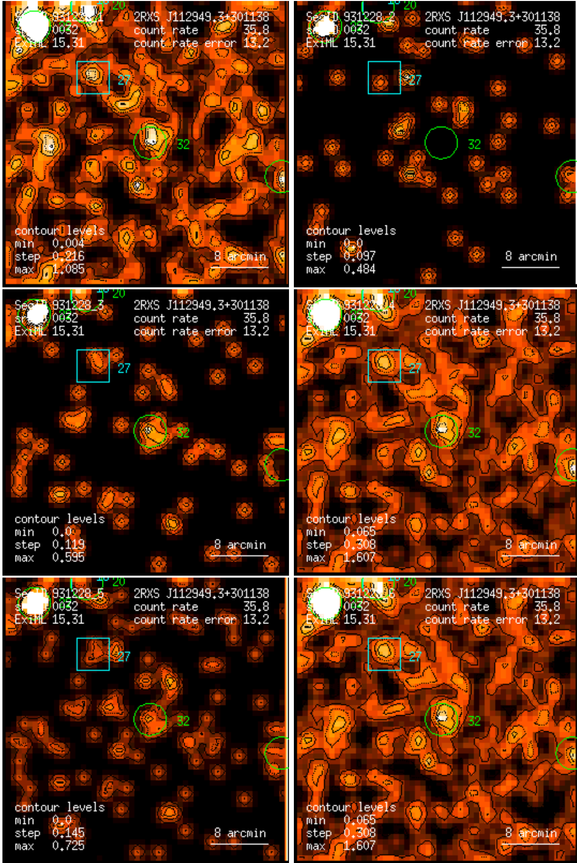
Figure 32: RASS 931228: detection 0032: band rate images, Gaussian filter: (1) PSPC channels 11 – 41, (2) 52 – 90, (3) 91 – 201, (4) 11 – 235, (5) 52 – 201, (6) 11 – 201. Broad band rates in counts/ks. Band rate contour levels in counts/ks/arcmin 2 .
