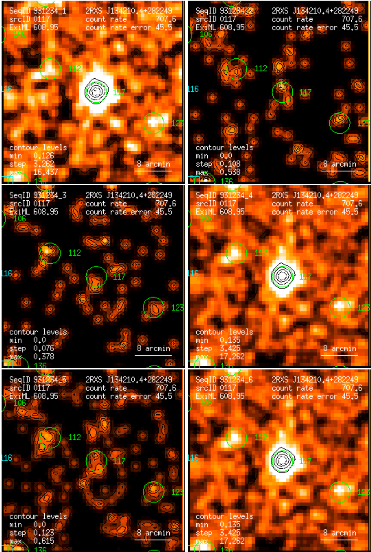
Figure 117: RASS 931234: detection 0117: band rate images, Gaussian filter: (1) PSPC channels 11 – 41, (2) 52 – 90, (3) 91 – 201, (4) 11 – 235, (5) 52 – 201, (6) 11 – 201. Broad band rates in counts/ks. Band rate contour levels in counts/ks/arcmin 2 .
