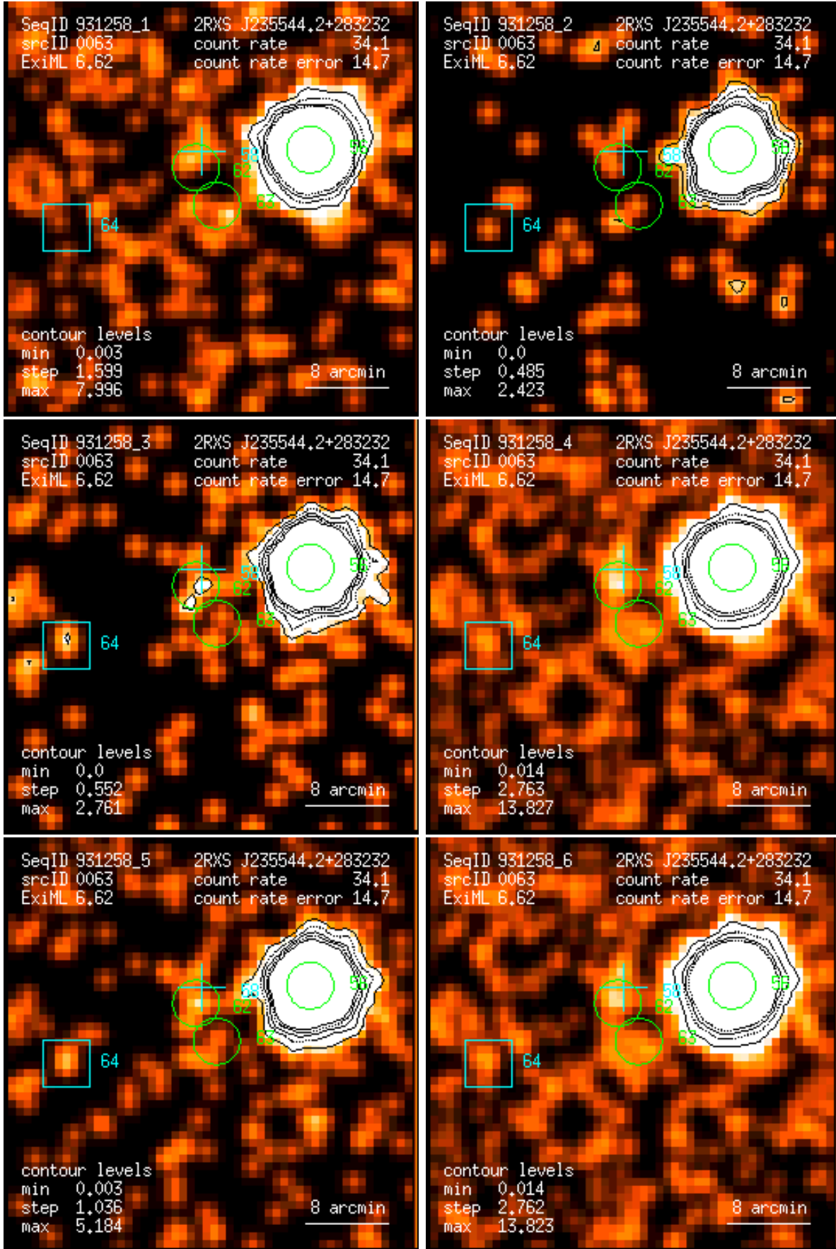
Figure 63: RASS 931258: detection 0063: band rate images, Gaussian filter: (1) PSPC channels 11 – 41, (2) 52 – 90, (3) 91 – 201, (4) 11 – 235, (5) 52 – 201, (6) 11 – 201. Broad band rates in counts/ks. Band rate contour levels in counts/ks/arcmin 2 .
