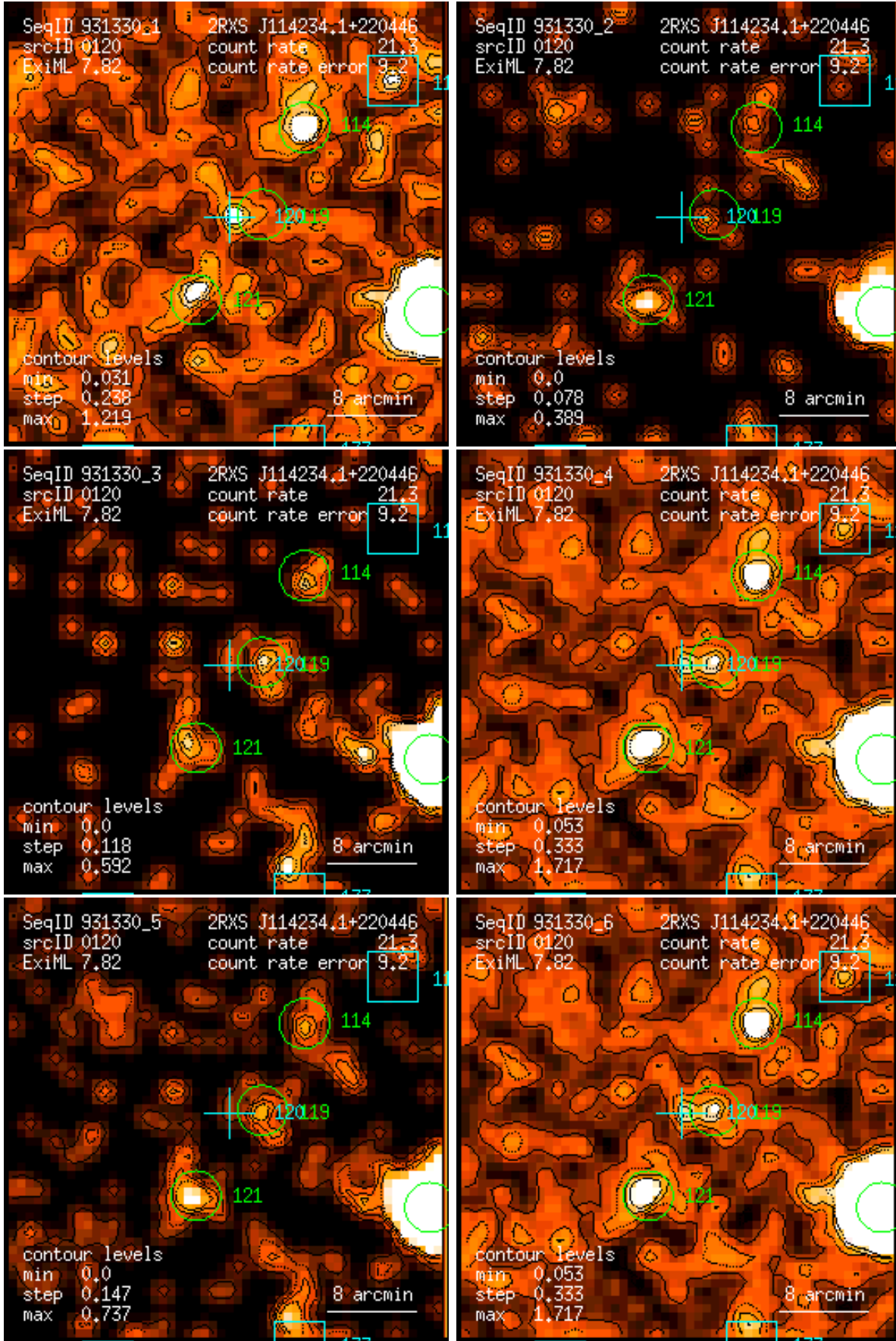
Figure 120: RASS 931330: detection 0120: band rate images, Gaussian filter: (1) PSPC channels 11 – 41, (2) 52 – 90, (3) 91 – 201, (4) 11 – 235, (5) 52 – 201, (6) 11 – 201. Broad band rates in counts/ks. Band rate contour levels in counts/ks/arcmin 2 .
