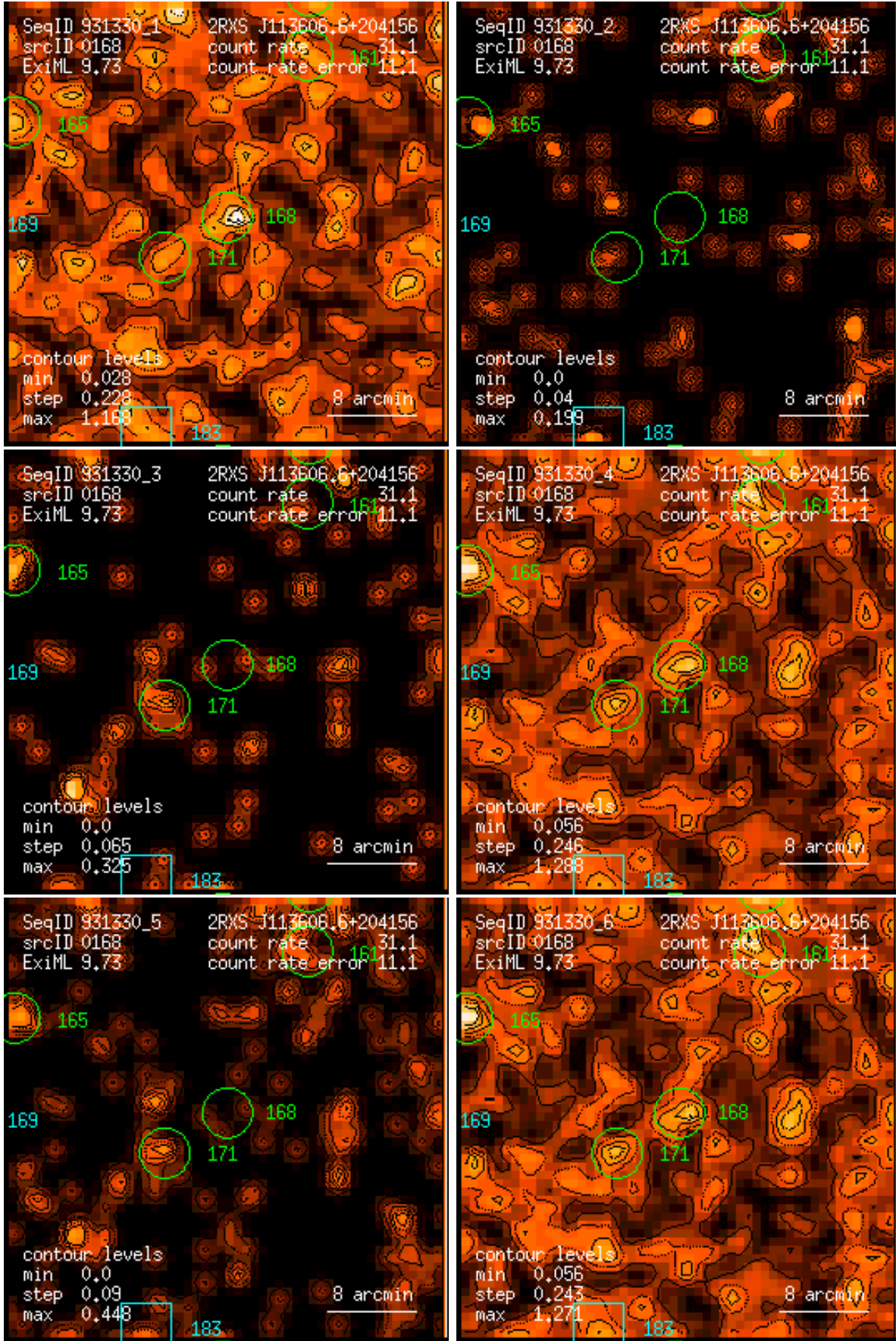
Figure 168: RASS 931330: detection 0168: band rate images, Gaussian filter: (1) PSPC channels 11 – 41, (2) 52 – 90, (3) 91 – 201, (4) 11 – 235, (5) 52 – 201, (6) 11 – 201. Broad band rates in counts/ks. Band rate contour levels in counts/ks/arcmin 2 .
