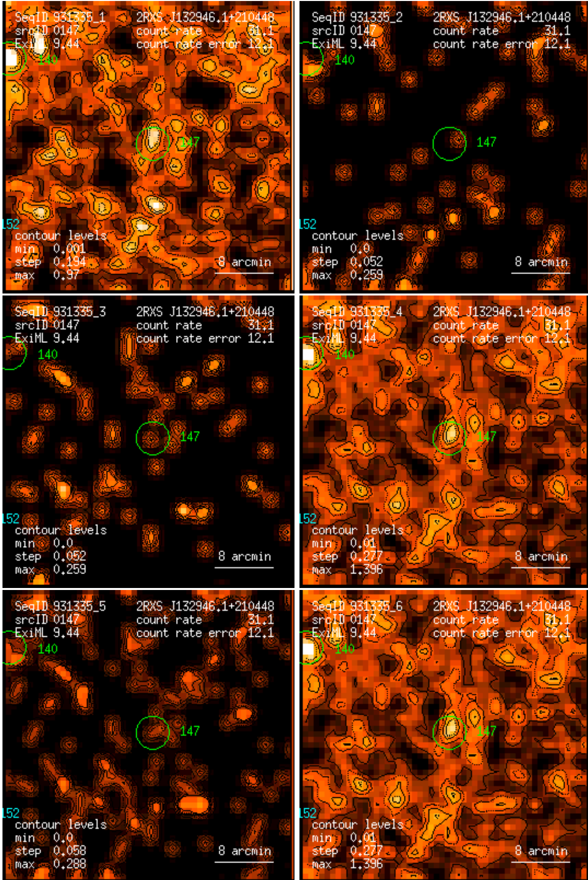
Figure 147: RASS 931335: detection 0147: band rate images, Gaussian filter: (1) PSPC channels 11 – 41, (2) 52 – 90, (3) 91 – 201, (4) 11 – 235, (5) 52 – 201, (6) 11 – 201. Broad band rates in counts/ks. Band rate contour levels in counts/ks/arcmin 2 .
