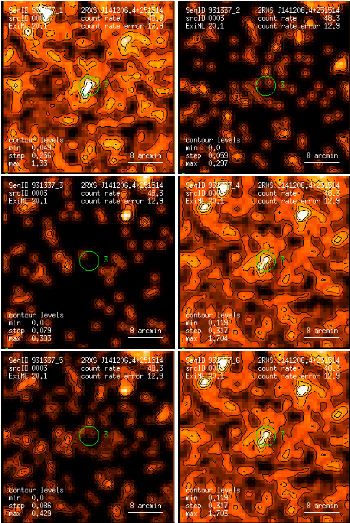
Figure 3: RASS 931337: detection 0003: band rate images, Gaussian filter: (1) PSPC channels 11 – 41, (2) 52 – 90, (3) 91 – 201, (4) 11 – 235, (5) 52 – 201, (6) 11 – 201. Broad band rates in counts/ks. Band rate contour levels in counts/ks/arcmin 2 .
