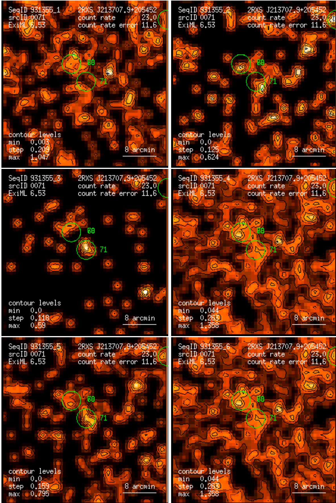
Figure 71: RASS 931355: detection 0071: band rate images, Gaussian filter: (1) PSPC channels 11 – 41, (2) 52 – 90, (3) 91 – 201, (4) 11 – 235, (5) 52 – 201, (6) 11 – 201. Broad band rates in counts/ks. Band rate contour levels in counts/ks/arcmin 2 .
