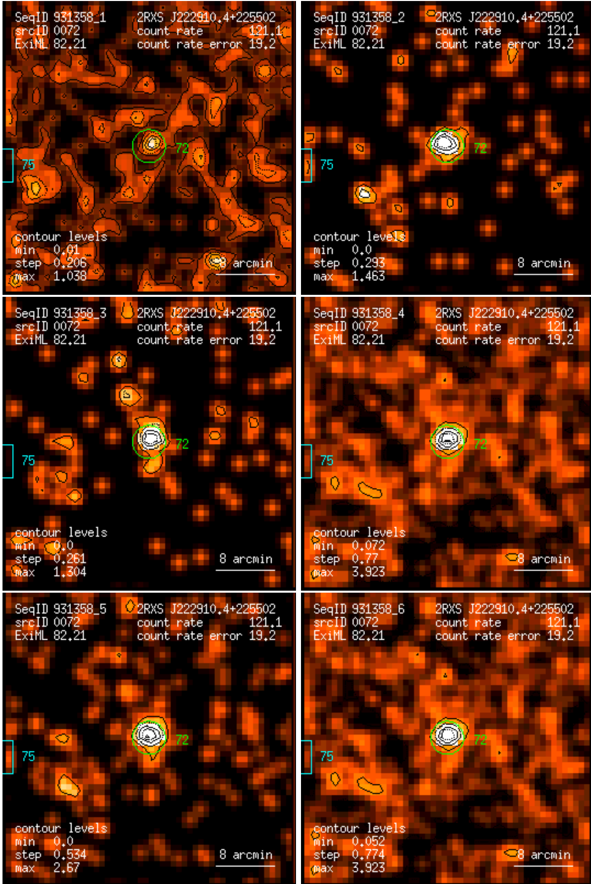
Figure 72: RASS 931358: detection 0072: band rate images, Gaussian filter: (1) PSPC channels 11 – 41, (2) 52 – 90, (3) 91 – 201, (4) 11 – 235, (5) 52 – 201, (6) 11 – 201. Broad band rates in counts/ks. Band rate contour levels in counts/ks/arcmin 2 .
