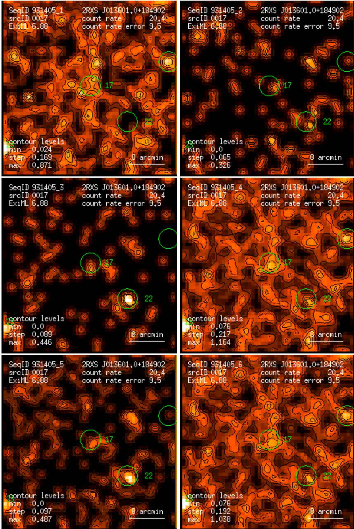
Figure 17: RASS 931405: detection 0017: band rate images, Gaussian filter: (1) PSPC channels 11 – 41, (2) 52 – 90, (3) 91 – 201, (4) 11 – 235, (5) 52 – 201, (6) 11 – 201. Broad band rates in counts/ks. Band rate contour levels in counts/ks/arcmin 2 .
