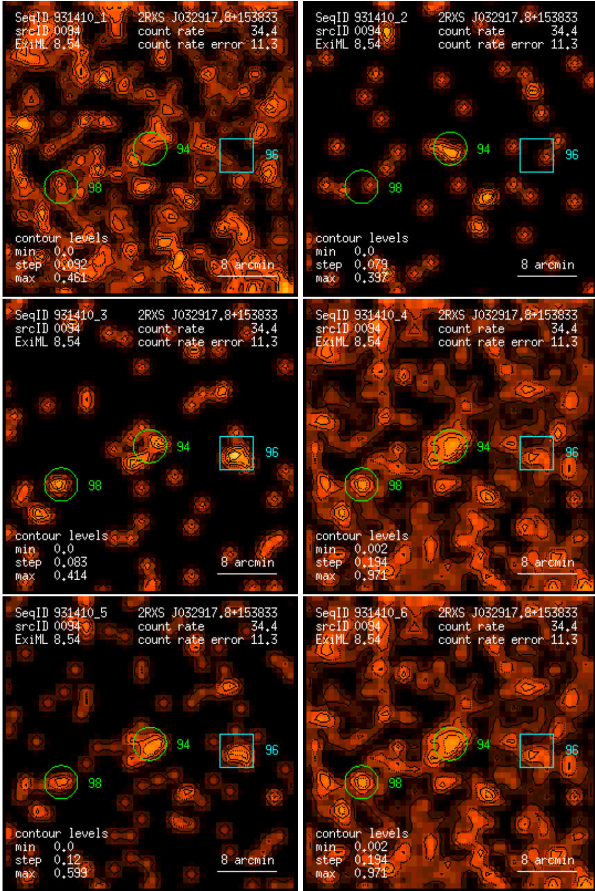
Figure 94: RASS 931410: detection 0094: band rate images, Gaussian filter: (1) PSPC channels 11 – 41, (2) 52 – 90, (3) 91 – 201, (4) 11 – 235, (5) 52 – 201, (6) 11 – 201. Broad band rates in counts/ks. Band rate contour levels in counts/ks/arcmin 2 .
