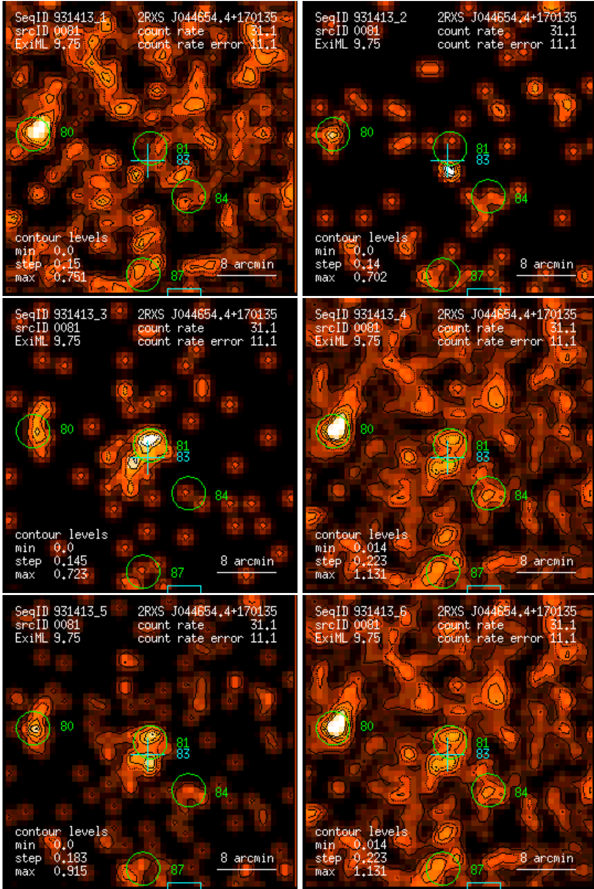
Figure 81: RASS 931413: detection 0081: band rate images, Gaussian filter: (1) PSPC channels 11 – 41, (2) 52 – 90, (3) 91 – 201, (4) 11 – 235, (5) 52 – 201, (6) 11 – 201. Broad band rates in counts/ks. Band rate contour levels in counts/ks/arcmin 2 .
