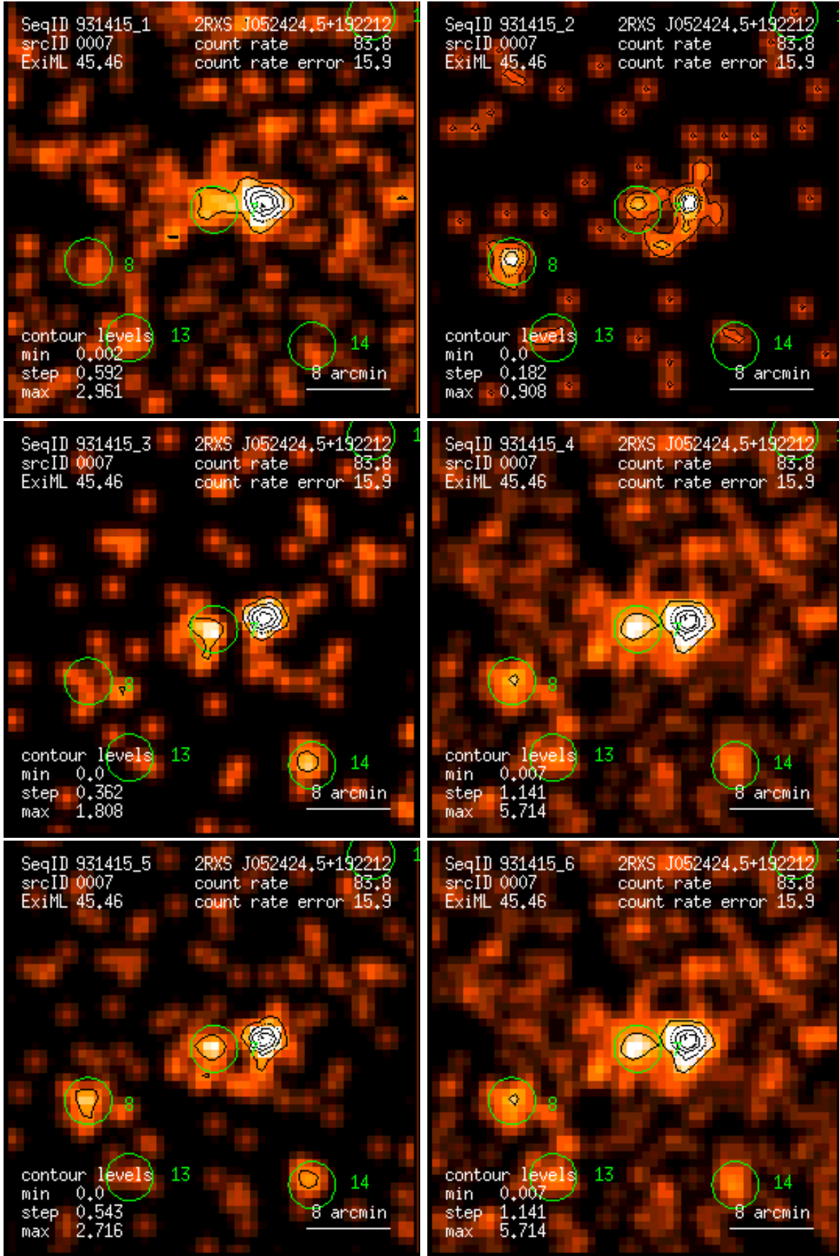
Figure 7: RASS 931415: detection 0007: band rate images, Gaussian filter: (1) PSPC channels 11 – 41, (2) 52 – 90, (3) 91 – 201, (4) 11 – 235, (5) 52 – 201, (6) 11 – 201. Broad band rates in counts/ks. Band rate contour levels in counts/ks/arcmin 2 .
