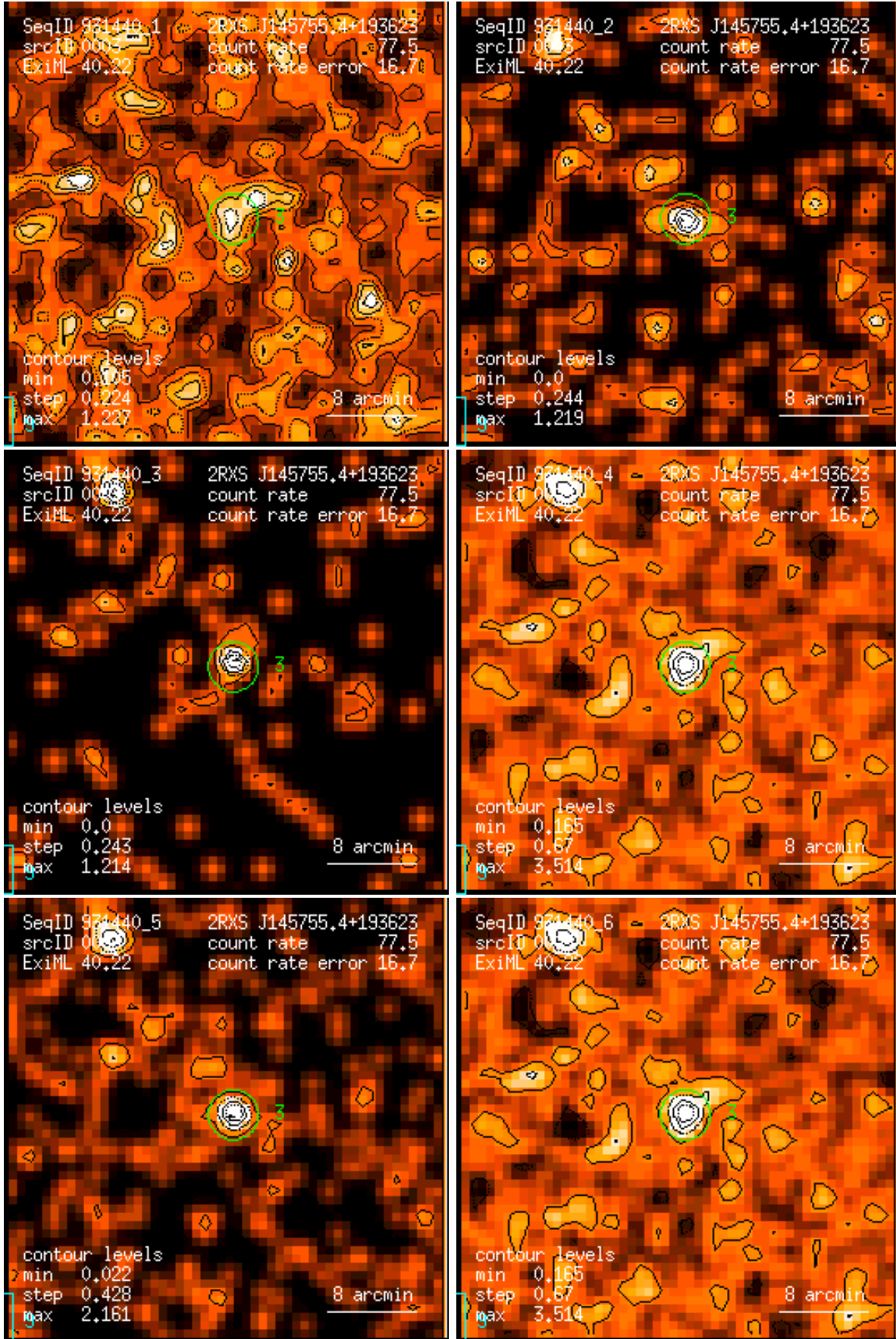
Figure 3: RASS 931440: detection 0003: band rate images, Gaussian filter: (1) PSC channels 11 – 41, (2) 52 – 90, (3) 91 – 201, (4) 11 – 235, (5) 52 – 201, (6) 11 – 201. Broad band rates in counts/ks. Band rate contour levels in counts/ks/arcmin 2 .
