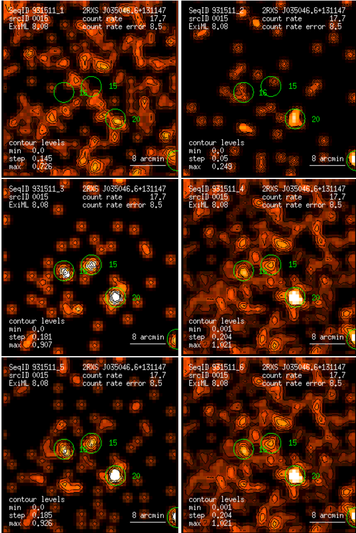
Figure 15: RASS 931511: detection 0015: band rate images, Gaussian filter: (1) PSPC channels 11 – 41, (2) 52 – 90, (3) 91 – 201, (4) 11 – 235, (5) 52 – 201, (6) 11 – 201. Broad band rates in counts/ks. Band rate contour levels in counts/ks/arcmin 2 .
