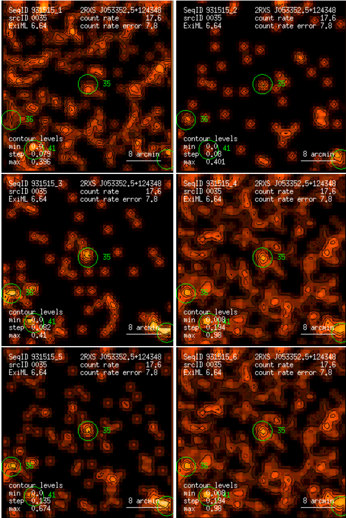
Figure 35: RASS 931515: detection 0035: band rate images, Gaussian filter: (1) PSPC channels 11 – 41, (2) 52 – 90, (3) 91 – 201, (4) 11 – 235, (5) 52 – 201, (6) 11 – 201. Broad band rates in counts/ks. Band rate contour levels in counts/ks/arcmin 2 .
