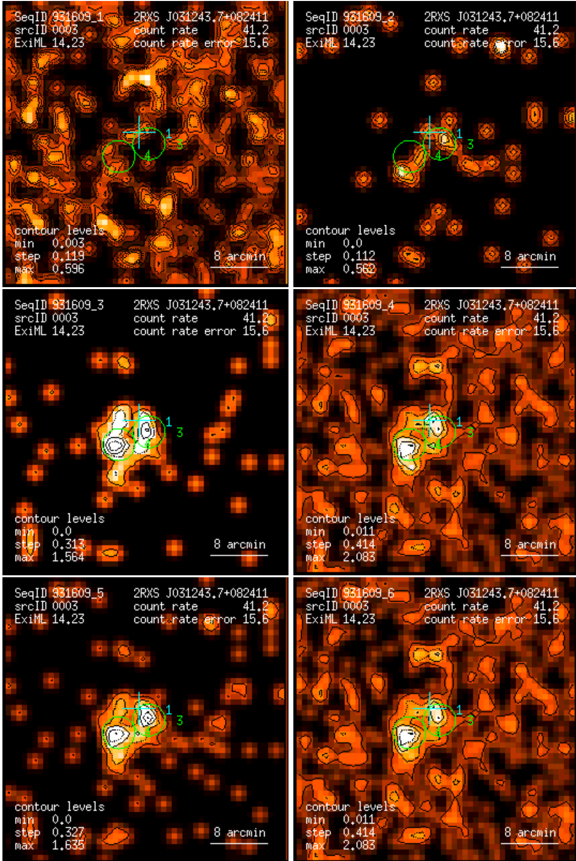
Figure 3: RASS 931609: detection 0003: band rate images, Gaussian filter: (1) PSPC channels 11 – 41, (2) 52 – 90, (3) 91 – 201, (4) 11 – 235, (5) 52 – 201, (6) 11 – 201. Broad band rates in counts/ks. Band rate contour levels in counts/ks/arcmin 2 .
