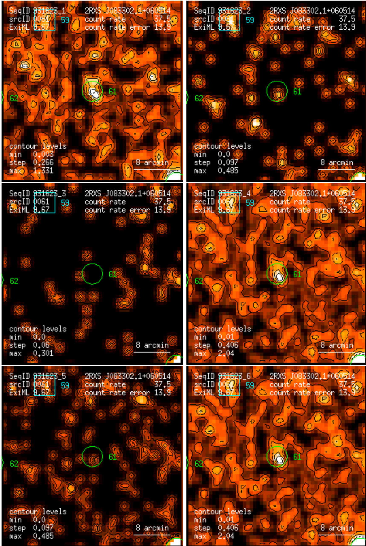
Figure 61: RASS 931623: detection 0061: band rate images, Gaussian filter: (1) PSPC channels 11 – 41, (2) 52 – 90, (3) 91 – 201, (4) 11 – 235, (5) 52 – 201, (6) 11 – 201. Broad band rates in counts/ks. Band rate contour levels in counts/ks/arcmin 2 .
