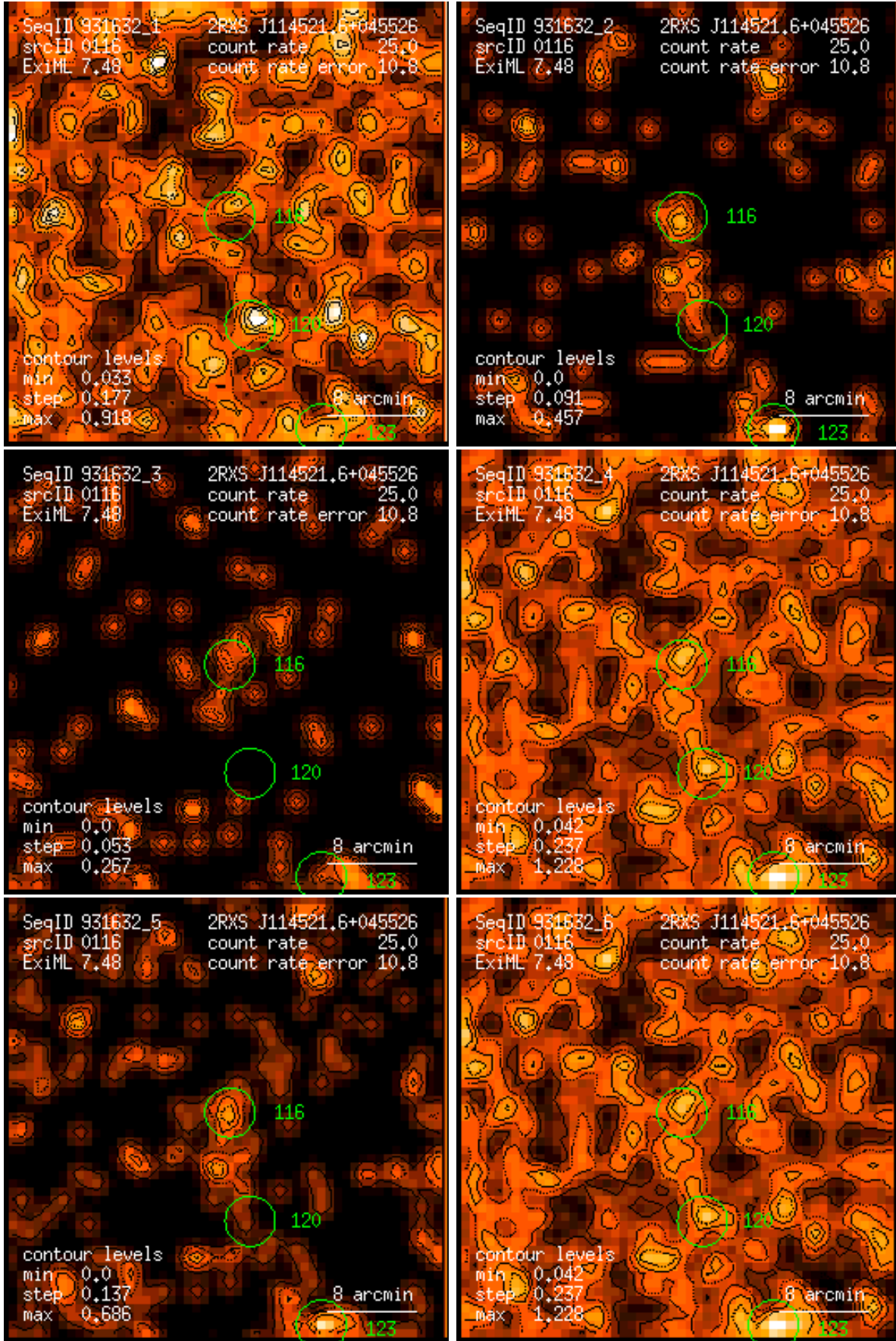
Figure 116: RASS 931632: detection 0116: band rate images, Gaussian filter: (1) PSPC channels 11 – 41, (2) 52 – 90, (3) 91 – 201, (4) 11 – 235, (5) 52 – 201, (6) 11 – 201. Broad band rates in counts/ks. Band rate contour levels in counts/ks/arcmin 2 .
