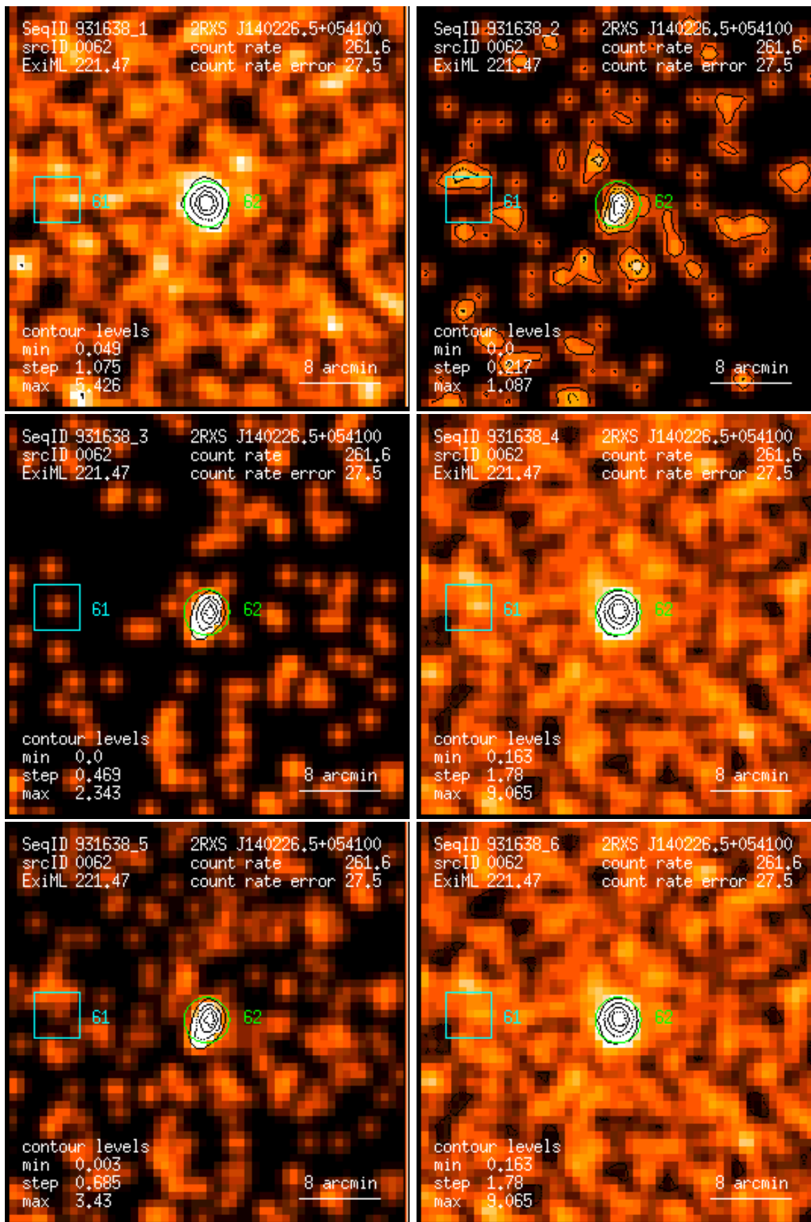
Figure 62: RASS 931638: detection 0062: band rate images, Gaussian filter: (1) PSPC channels 11 – 41, (2) 52 – 90, (3) 91 – 201, (4) 11 – 235, (5) 52 – 201, (6) 11 – 201. Broad band rates in counts/ks. Band rate contour levels in counts/ks/arcmin 2 .
