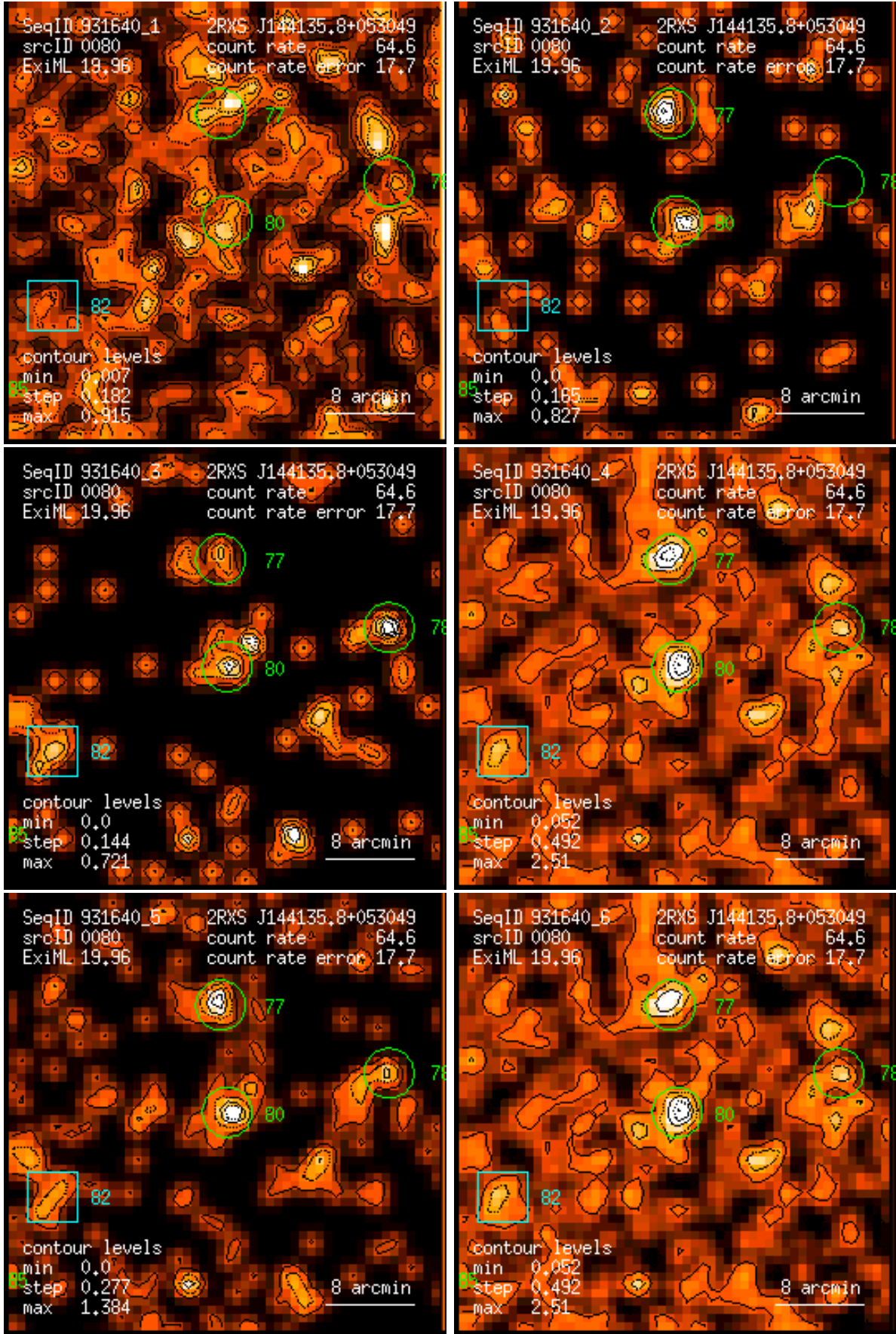
Figure 80: RASS 931640: detection 0080: band rate images, Gaussian filter: (1) PSPC channels 11 – 41, (2) 52 – 90, (3) 91 – 201, (4) 11 – 235, (5) 52 – 201, (6) 11 – 201. Broad band rates in counts/ks. Band rate contour levels in counts/ks/arcmin 2 .
