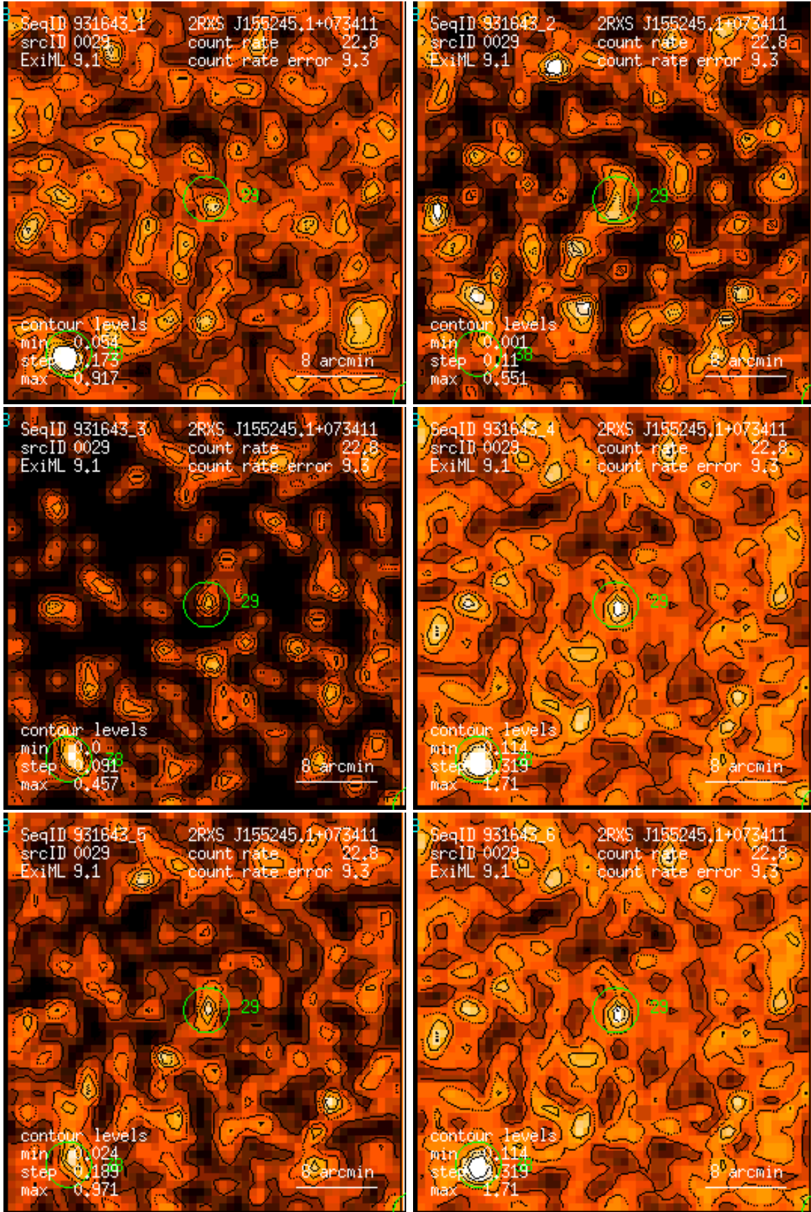
Figure 29: RASS 931643: detection 0029: band rate images, Gaussian filter: (1) PSPC channels 11 – 41, (2) 52 – 90, (3) 91 – 201, (4) 11 – 235, (5) 52 – 201, (6) 11 – 201. Broad band rates in counts/ks. Band rate contour levels in counts/ks/arcmin 2 .
