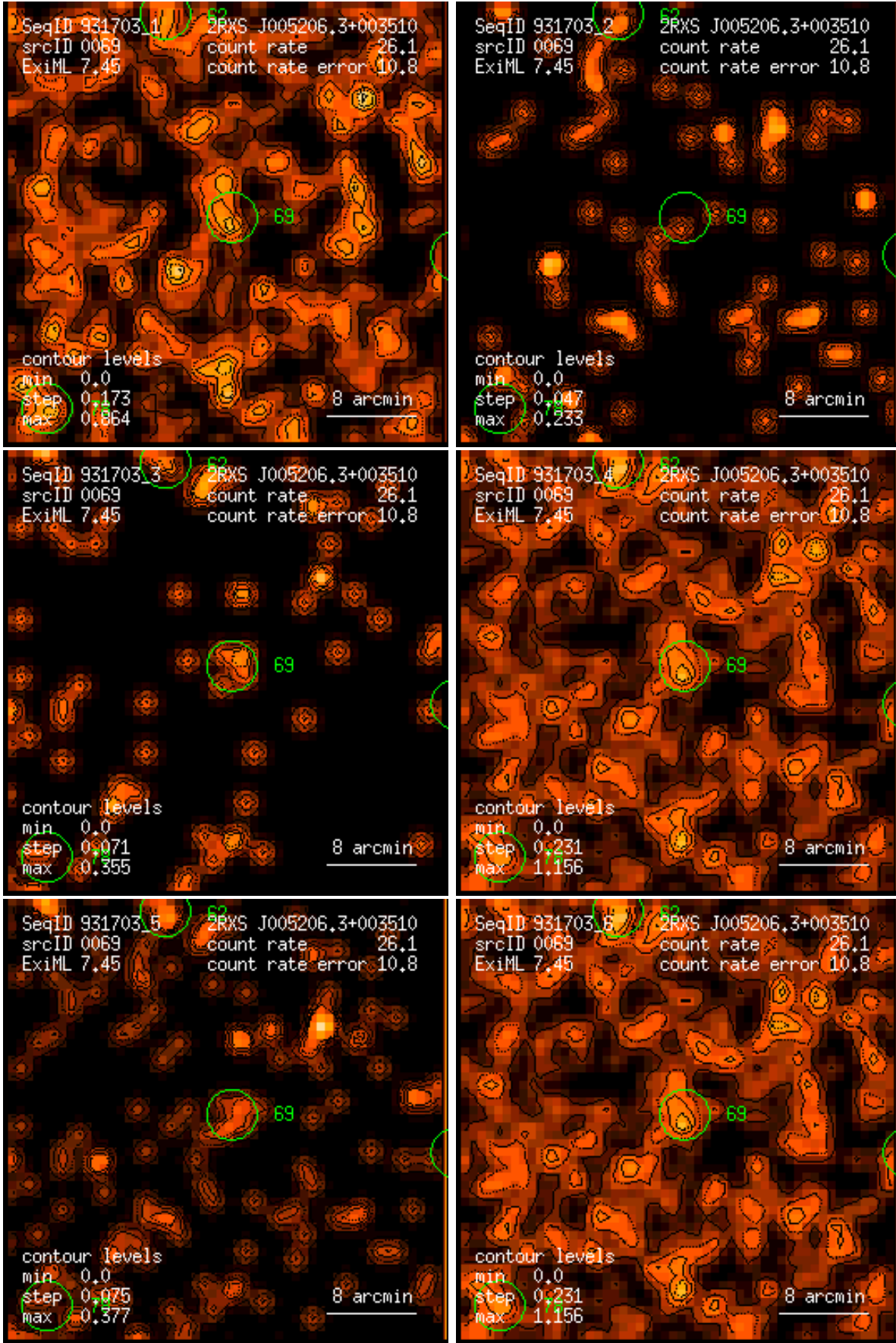
Figure 69: RASS 931703: detection 0069: band rate images, Gaussian filter: (1) PSPC channels 11 – 41, (2) 52 – 90, (3) 91 – 201, (4) 11 – 235, (5) 52 – 201, (6) 11 – 201. Broad band rates in counts/ks. Band rate contour levels in counts/ks/arcmin 2 .
