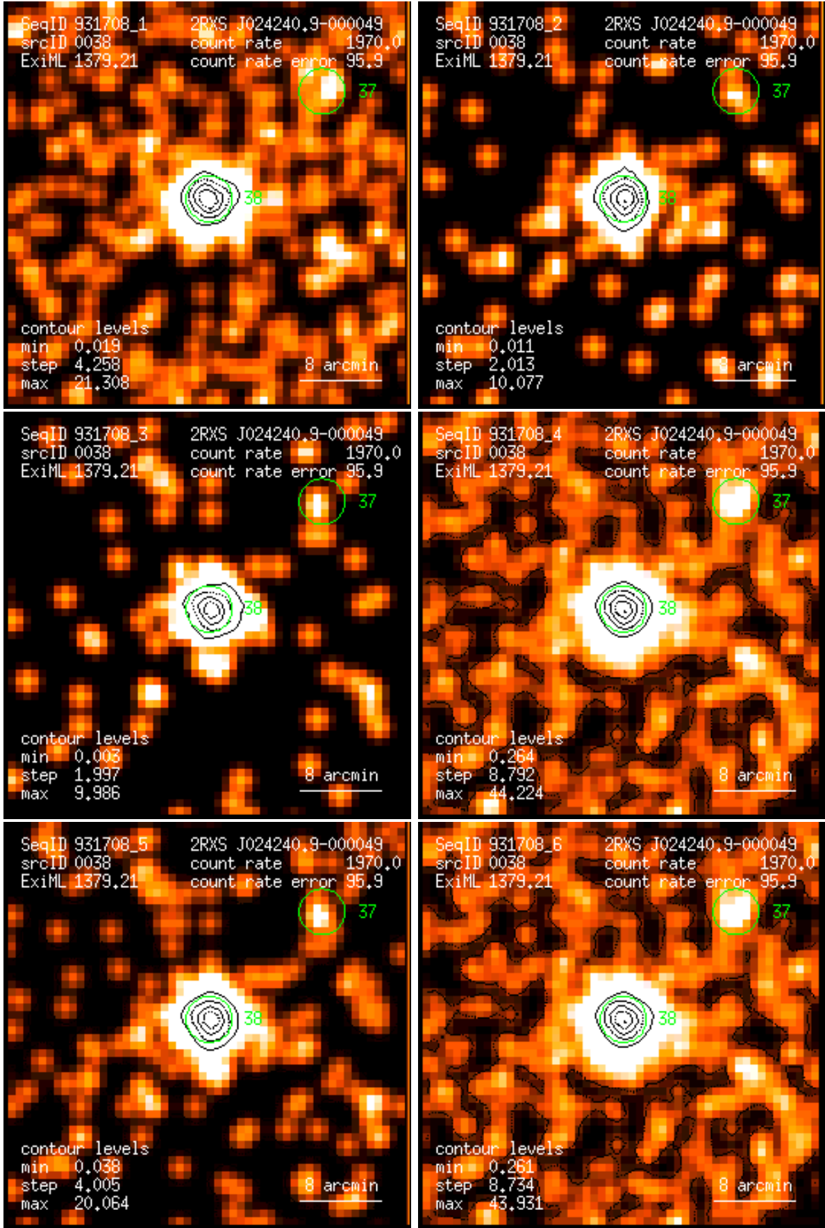
Figure 38: RASS 931708: detection 0038: band rate images, Gaussian filter: (1) PSPC channels 11 – 41, (2) 52 – 90, (3) 91 – 201, (4) 11 – 235, (5) 52 – 201, (6) 11 – 201. Broad band rates in counts/ks. Band rate contour levels in counts/ks/arcmin 2 .
