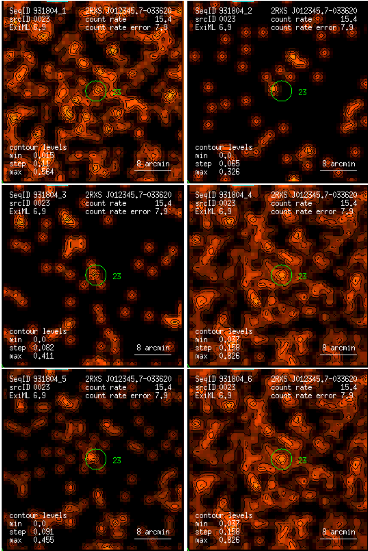
Figure 23: RASS 931804: detection 0023: band rate images, Gaussian filter: (1) PSPC channels 11 – 41, (2) 52 – 90, (3) 91 – 201, (4) 11 – 235, (5) 52 – 201, (6) 11 – 201. Broad band rates in counts/ks. Band rate contour levels in counts/ks/arcmin 2 .
